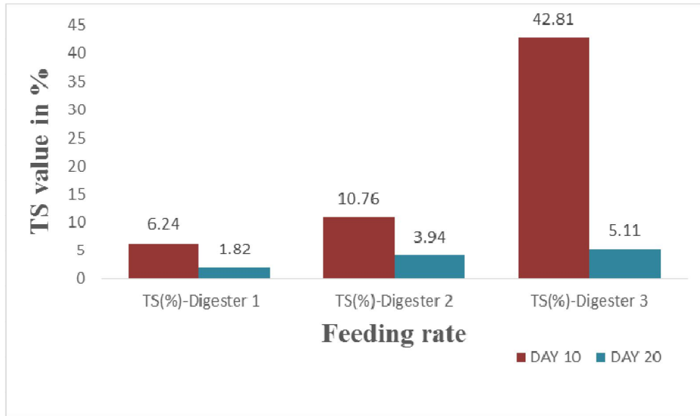
Figure 6: Variation of effluent total solid for digester 1 to 3
