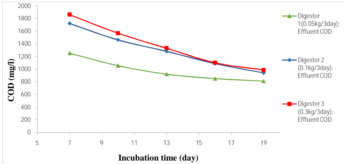
Figure 5: COD variation of effluent for digester 1 to 3
