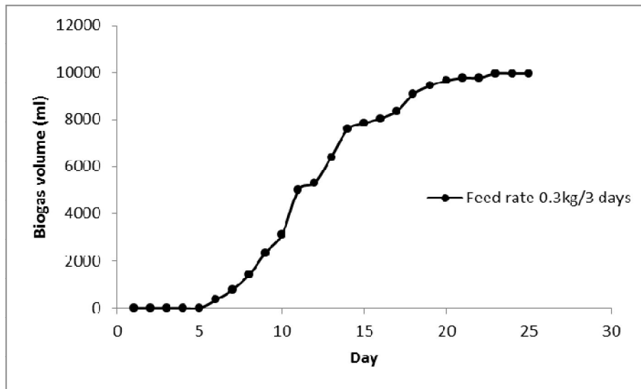
Figure 4: Biogas production at 0.3 kg/3 days feed rate
