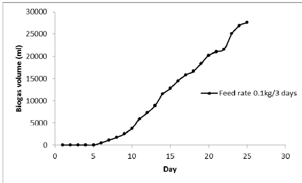
Figure 3: Biogas production at 0.1 kg/3 days feed rate
