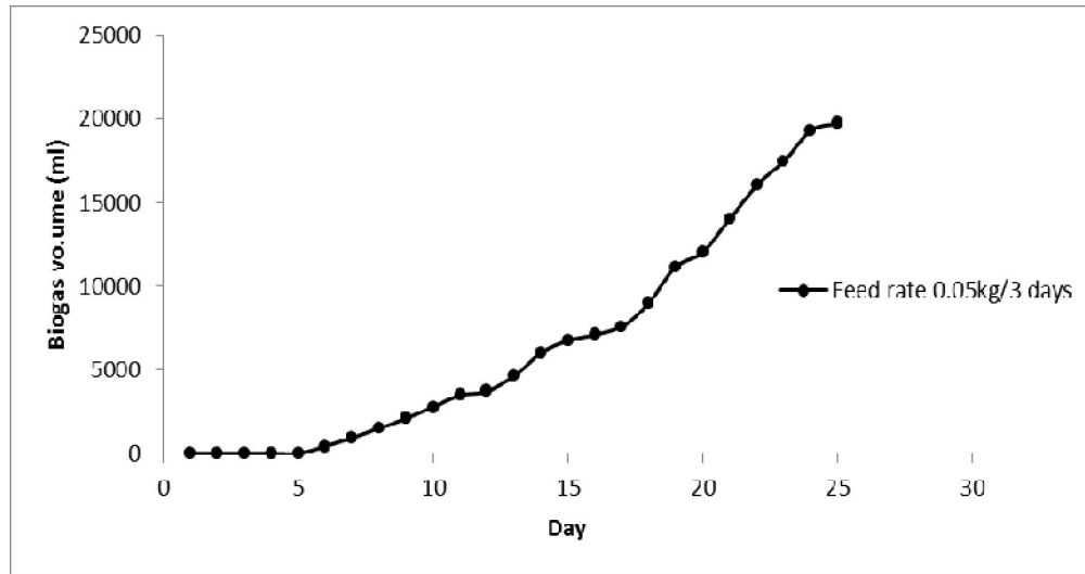
Figure 2: Biogas production at 0.05 kg/3 day feed rate
