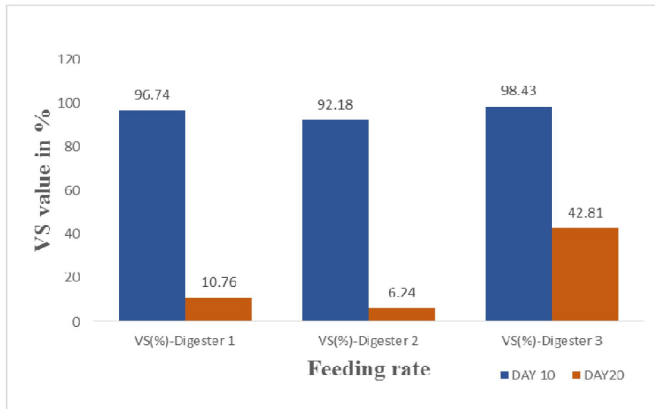
Figure 7: Volatile solid variation for three feed rate
