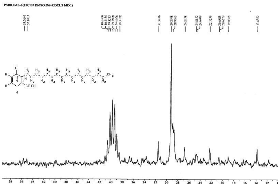
Fig. 4: ^{13}\text{C} NMR of 6-Heptadecylcyclohex -3-ene-1 carboxylic acid
