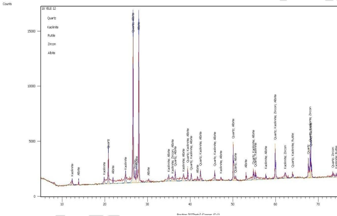
Fig 3.0: X-Ray Diffraction of sediment sample 18YELE 12 showing variation of minerals at different positions.
