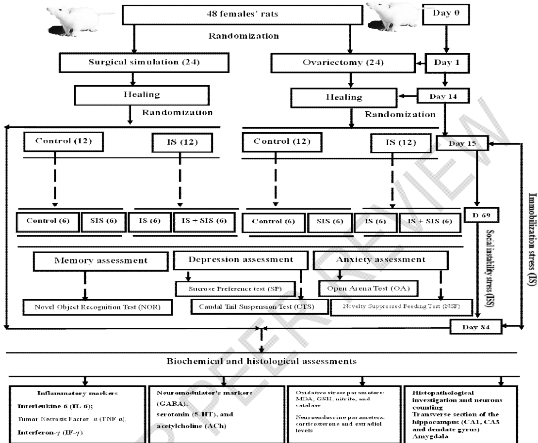
Figure 1: Experimental paradigm
