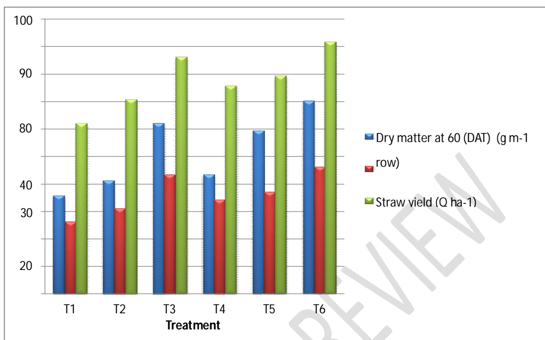
Fig-1 Effect of integrated use of chemical fertilizers, organic manure and bio-fertilizers on dry matter (g m -1 rowlength), grain and straw yield (Q ha -1 ) of rice crop
