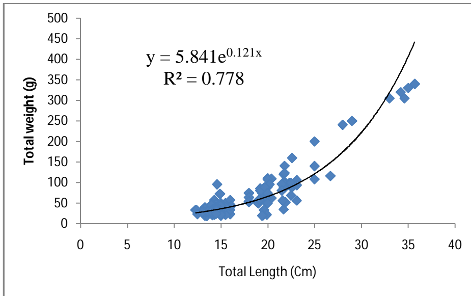
Figure 1: Length-weight relationship (LWR) of Schilbe mystis
