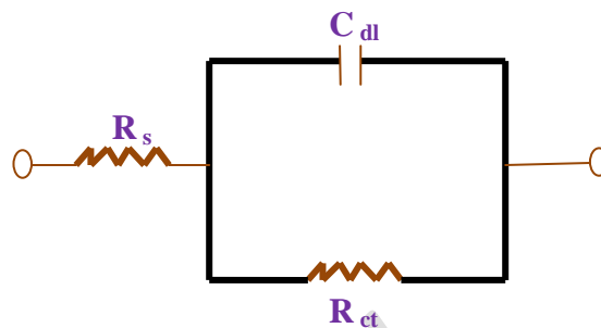
Fig. 3a: EIS equivalent Circuit
