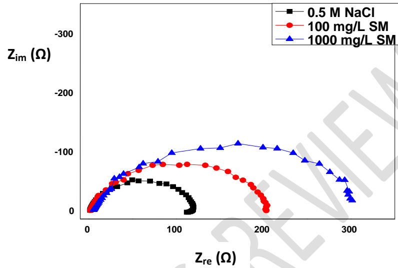
Fig 6: Nyquist plot of mild steel in 0.5 M NaCl environment in the presence and absence of SM
