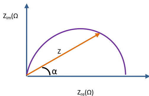
Fig. 3b: Nyquist plot with impedance vector (Z)
