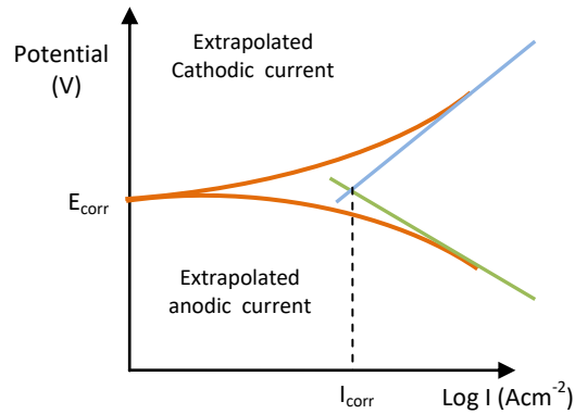
Fig. 2 Potentiodynamic polarization curves
