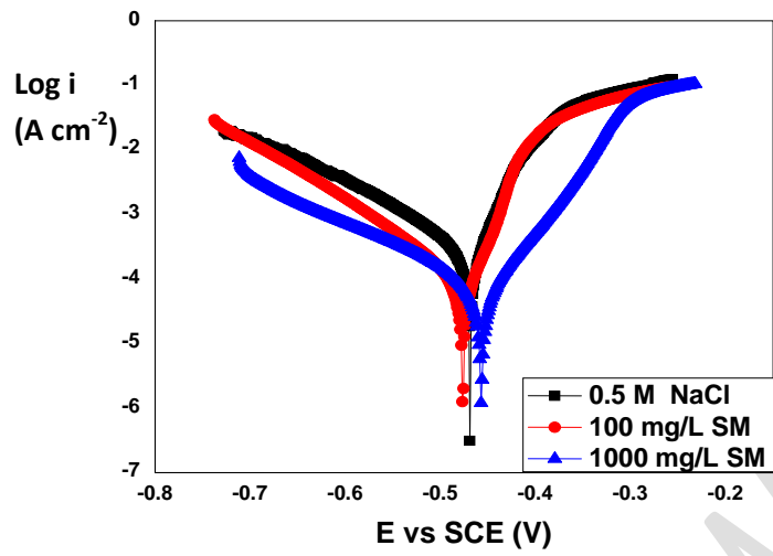
Fig. 4: Potentiodynamic polarization plot of mild steel in 0.5 M NaCl environment in the absence and presence of SM.
