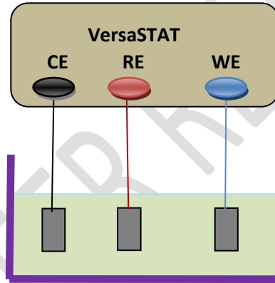
Fig. 1: The electrochemical measurements experimental setup with three-electrode
