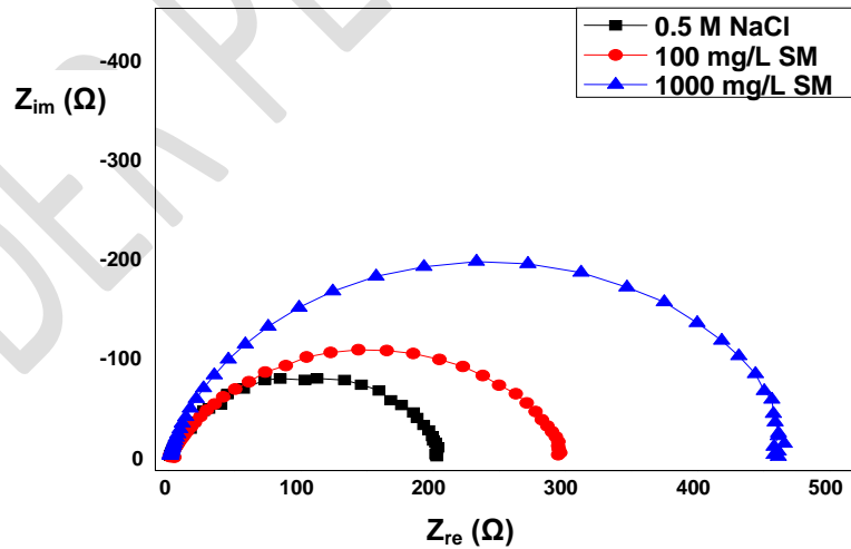
Fig 7: Nyquist plot of aluminium in 0.5 M NaCl environment in the presence and absence of SM
