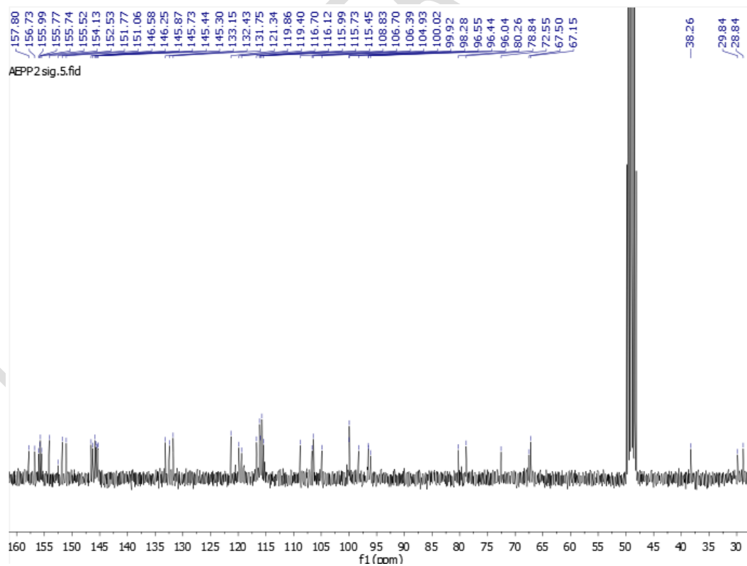
Figure 11 : ^{13}\text{C} NMR- spectrum of cinnamtannin B-1 (AJPP 3)
