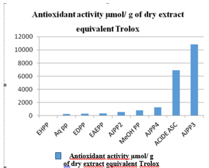
Figure 15: Diagram of the antioxidant activity of the different extracts and the molecule of Paullinia pinnata
