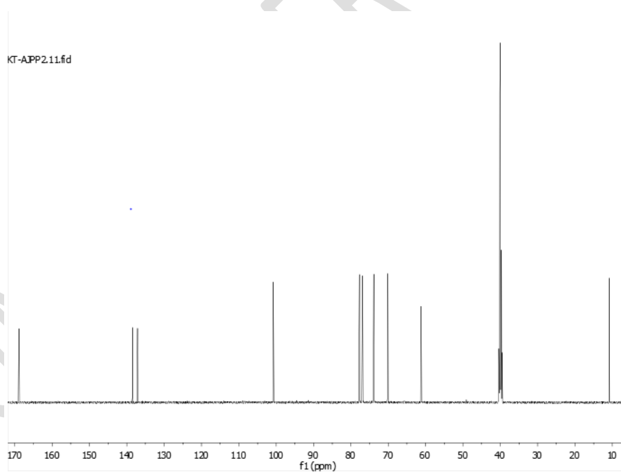
Figure 14 : ^{13}\text{C} NMR spectrum of O- \beta -D-glucopyranosyloxy-4-methyl-2 (5 H)-furanone
