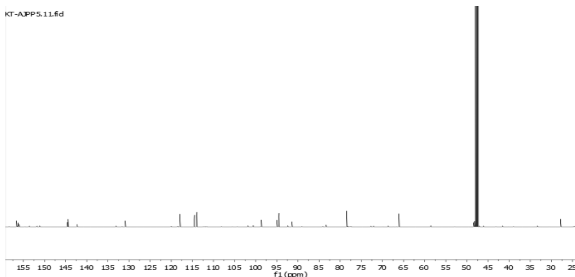
Figure 5 : ^{13}\text{C} -NMR Spectrum of epicatechin (AJPP 1)
