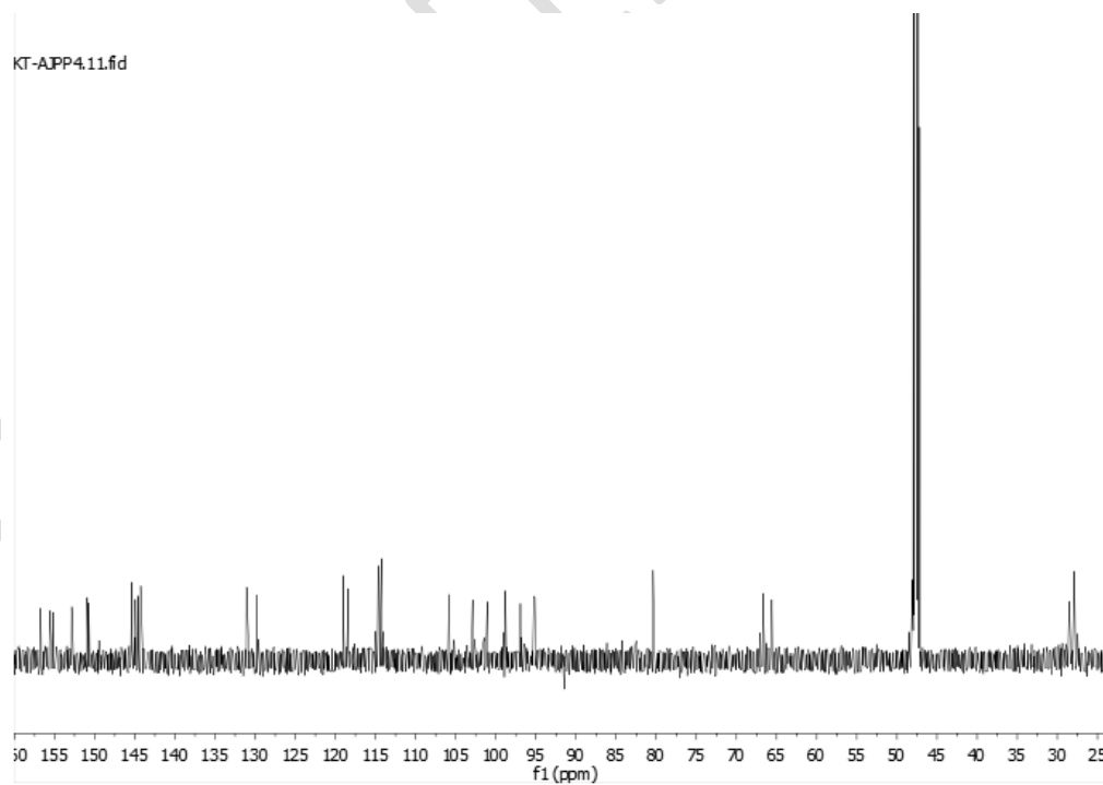
Figure 8: 13C NMR spectrum of proanthocyanidin A-2 (AJPP 2)
