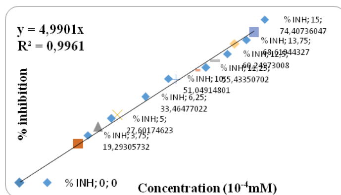
Figure 2: Trolox Calibration Curve (ABTS)
