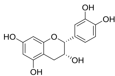
Figure 3: Structure of the molecule of epicatechin (AJPP 1)
