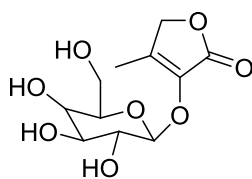
Figure 12 : Structure of the molecule of O- \beta\text{-D-glucopyranosyloxy}
