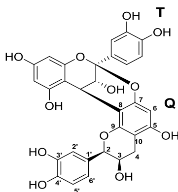
Figure 6 : Structure of the molecule of proanthocyanidin A-2 (AJPP 2)
