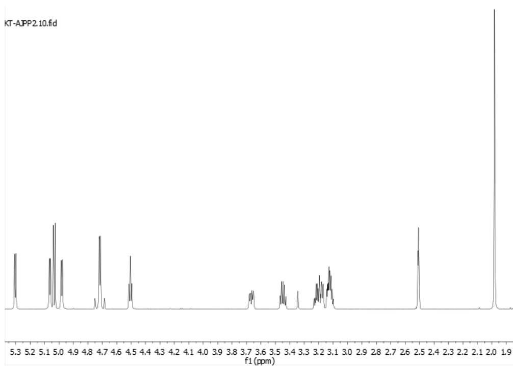
Figure 13 : ^1\text{H} NMR spectrum of O- \beta -D-glucopyranosyloxy-4-methyl-2 (5 H)-furanone
