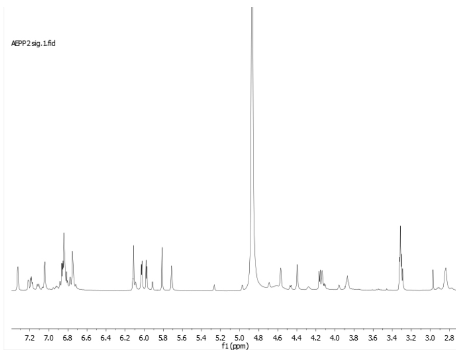
Figure 10: ^1\text{H} NMR- spectrum of cinnamtannin B-1 (AJPP 3)
