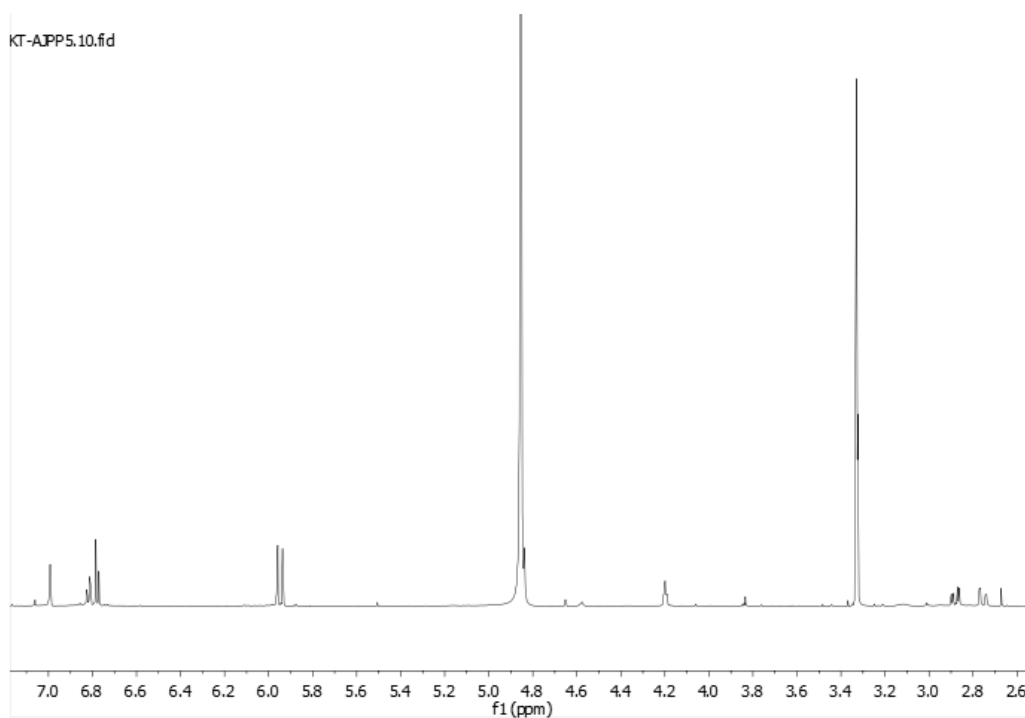
Figure 4: 1 H-NMR Spectrum of epicatechin (AJPP 1)
