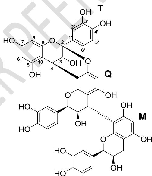
Figure 9 : Structure of the molecule of cinnamtannin B-1
