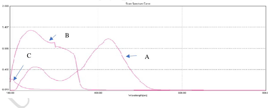
Figure 4. Absorption spectra
