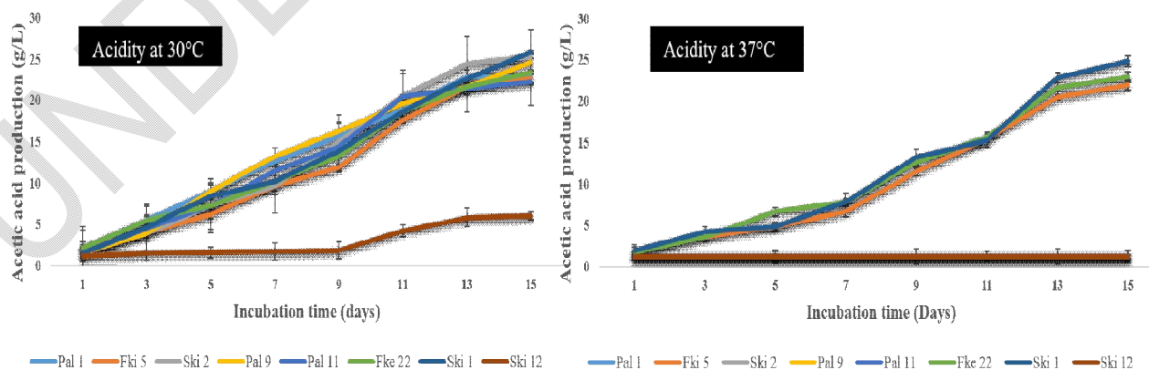
Figure 2: Effect of temperature on acetic acid yield by the 8 selected AAB with no overoxidation capacity.
