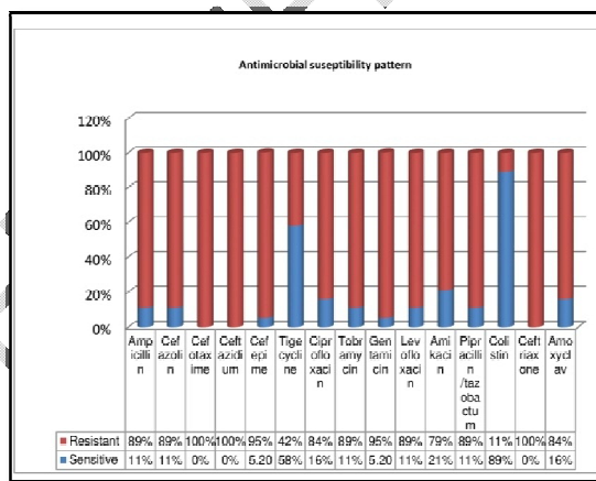
Fig 2. Antimicrobial susceptibility test
