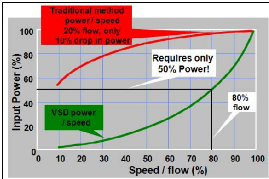
Figure 6: Relationships motor's power and motor's speed with and without a variable speed drive
