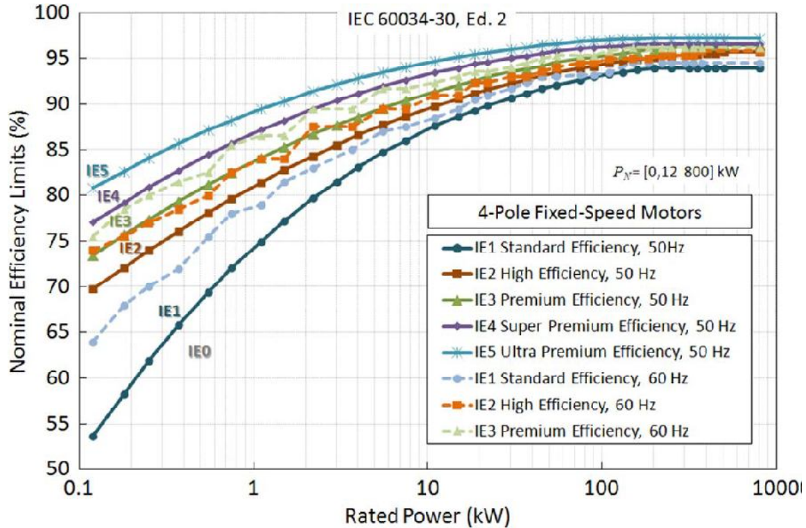
Figure 5: IEC 60034-30 nominal efficiency class limits, for four-pole motors [22]
