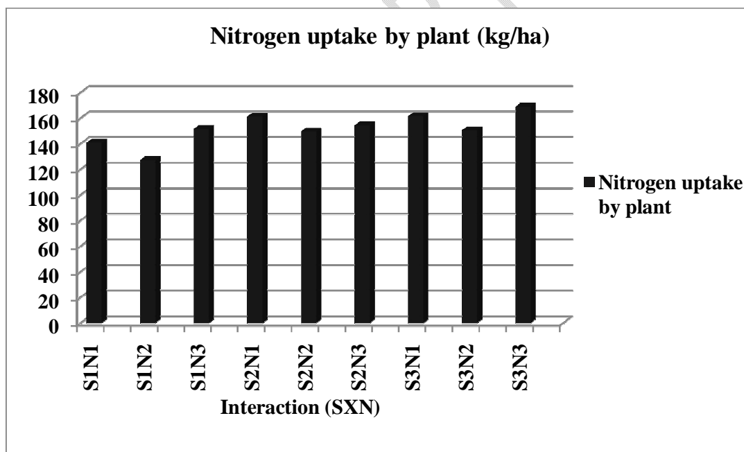
Figure 4. Effect of levels of spacing, nutrition and their interaction on Nitrogen uptake by the broccoli
