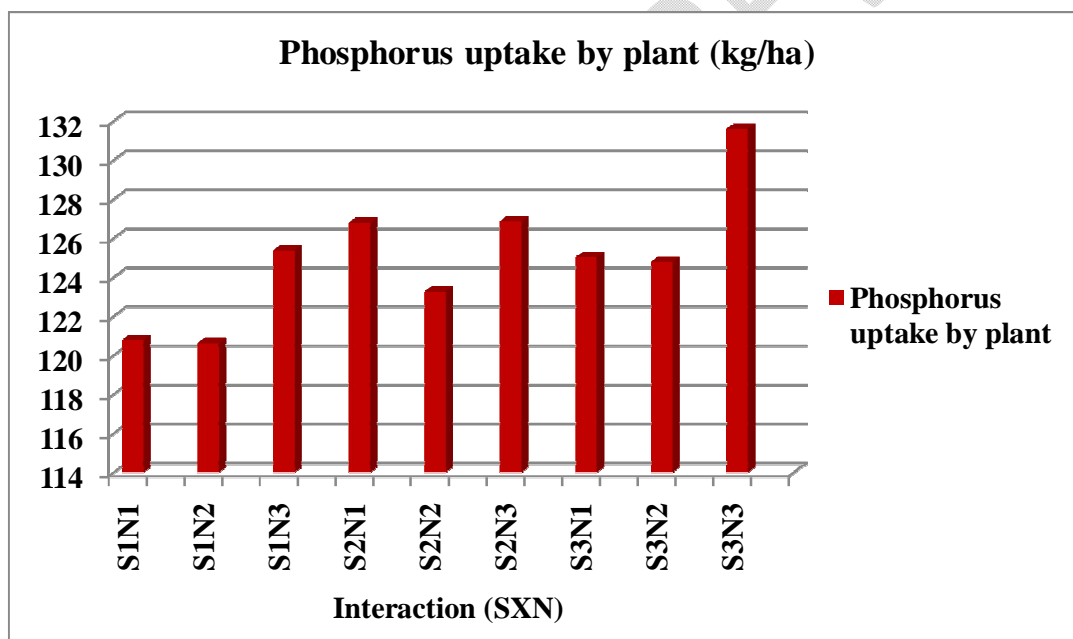
Figure 5. Effect of levels of spacing, nutrition and their interaction effect on Phosphorus uptake by the broccoli
