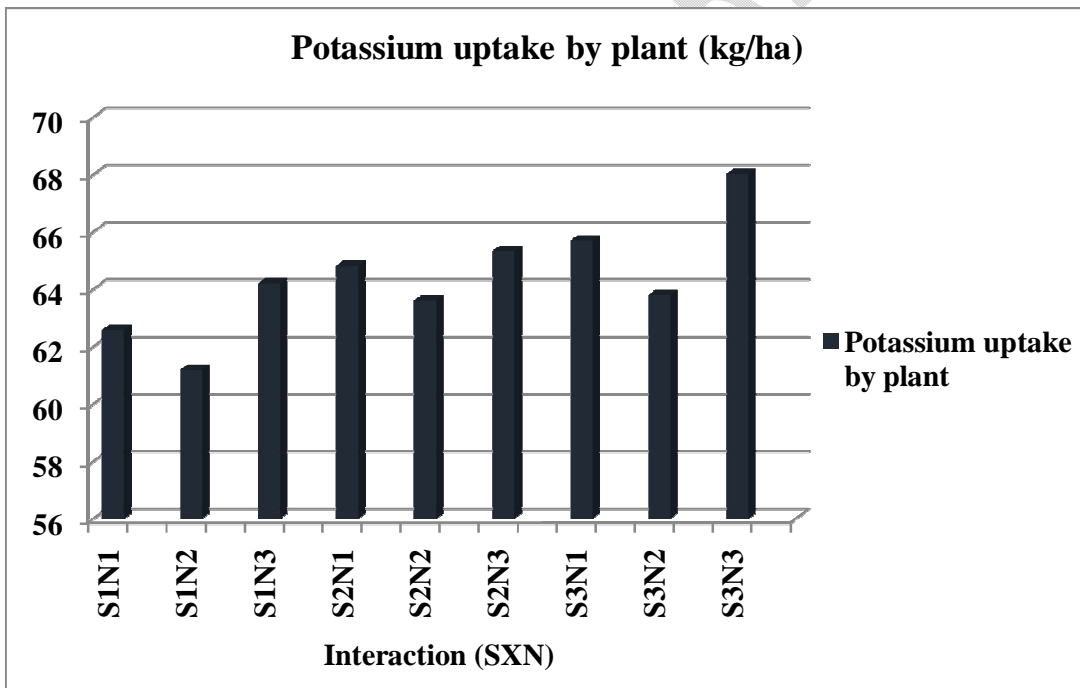
Figure 6. Effect of levels of spacing, nutrition and their interaction on Potassium uptake by the broccoli
