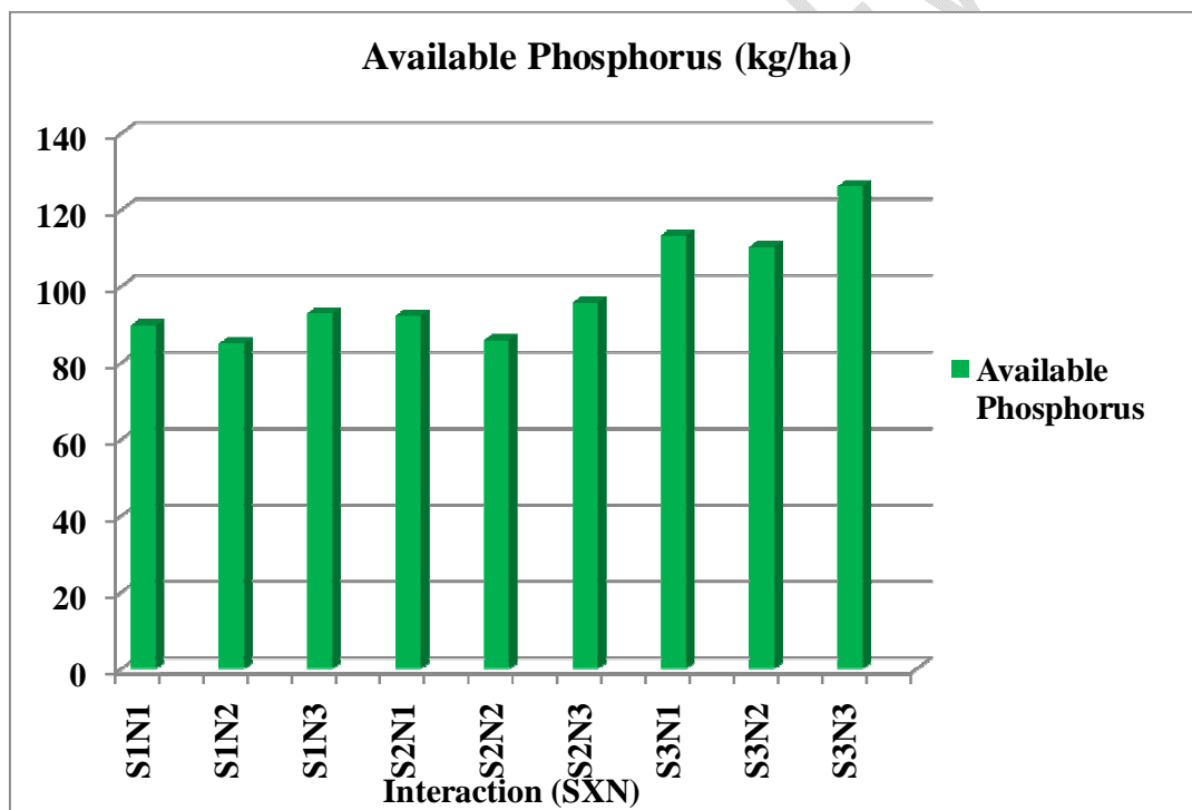
Figure 2. Effect of various levels of spacing, nutrient and their interaction on available Phosphorus
