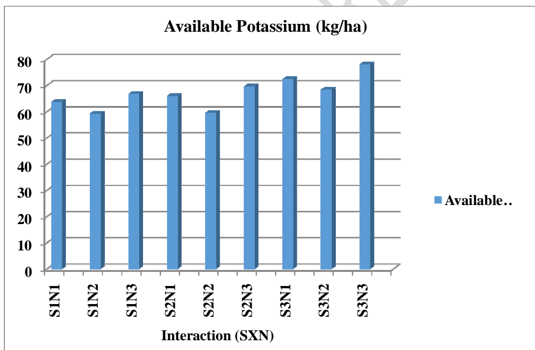
Figure. 3. Effect of various levels of spacing, nutrient and their interaction effect on available Potassium
