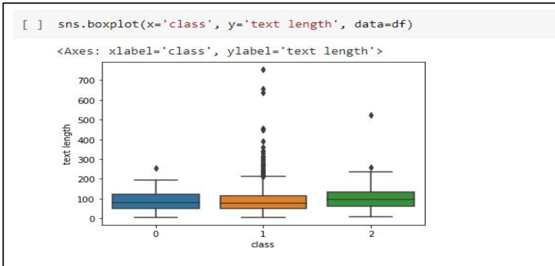
Fig 5. Box-plot visualization
