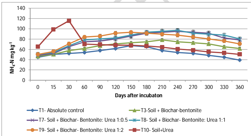
Fig 2: \text{NH}_4\text{-N} release from biochar and biochar blended urea fertilizers in sandy soils
