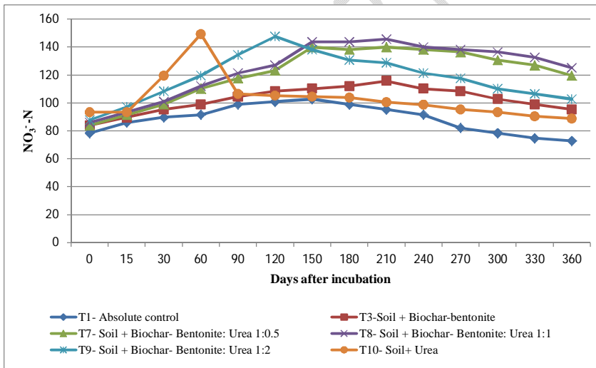
Fig 4: \text{NO}_3^- -N release from biochar and biochar blended urea fertilizers in sandy soil
