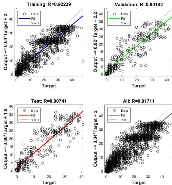
Figure 11. The fitting results of BP neural network optimized by genetic algorithm
