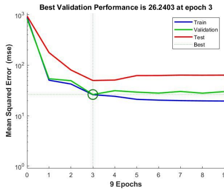
Figure 6. Training performance of neural networks
