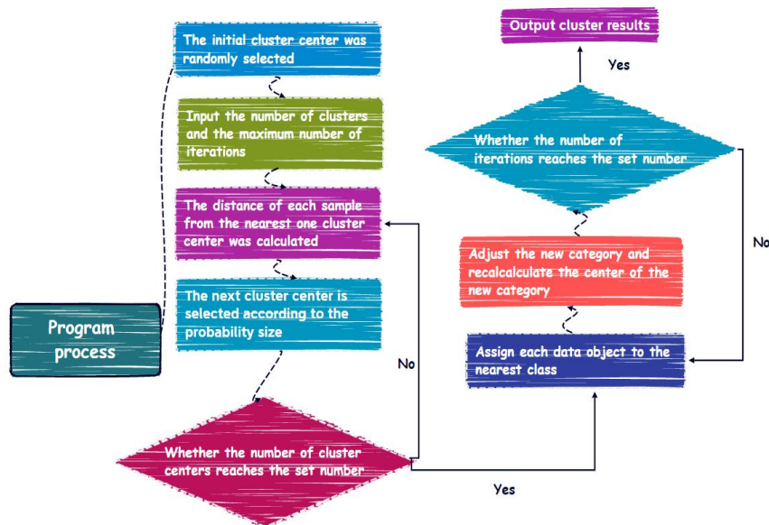
Figure 12. K-means cluster analysis flowchart
