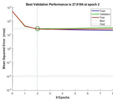
Figure 9. BP neural network training effect
