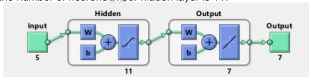
Figure 4. Schematic diagram of neural network structure
