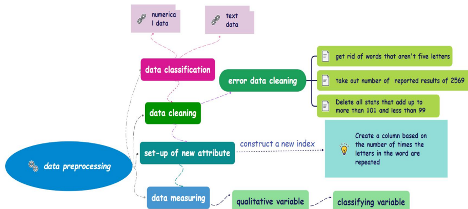
Figure 1 data preprocessing
