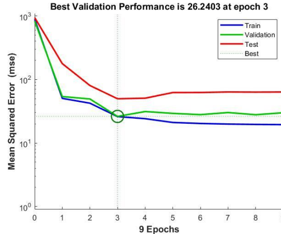
Figure 6. Training performance of neural networks
