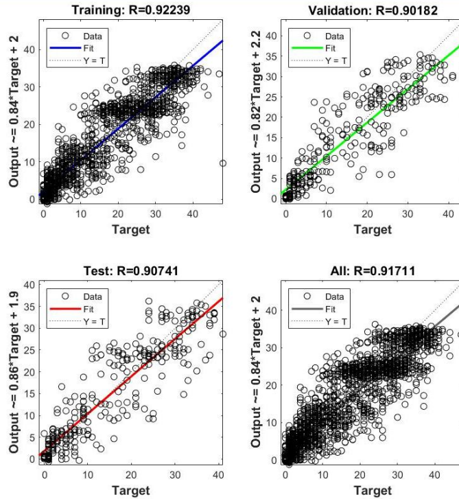
Figure 11. The fitting results of BP neural network optimized by genetic algorithm
