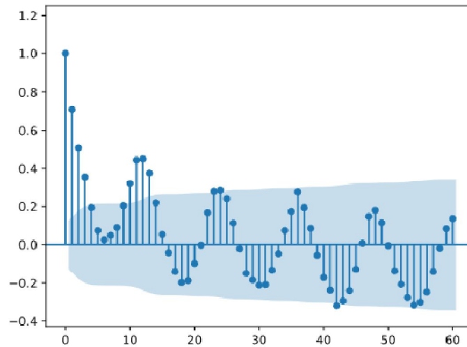
Fig. 2. Autocorrelation graph (xlabel:LAG, ylabel:autocorrelation)
