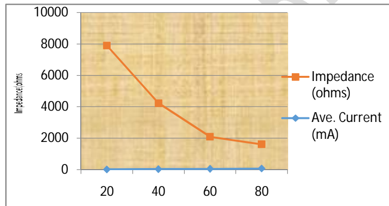
Figure 2: Graph of impedance vs. current levels on subject B
