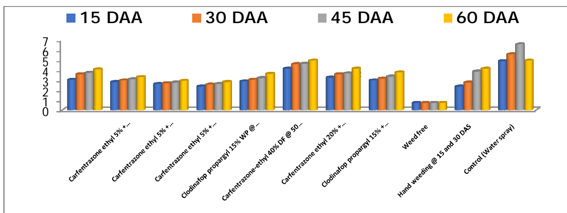
Fig.1: Phalaris minor density/m 2 after spraying of herbicides
