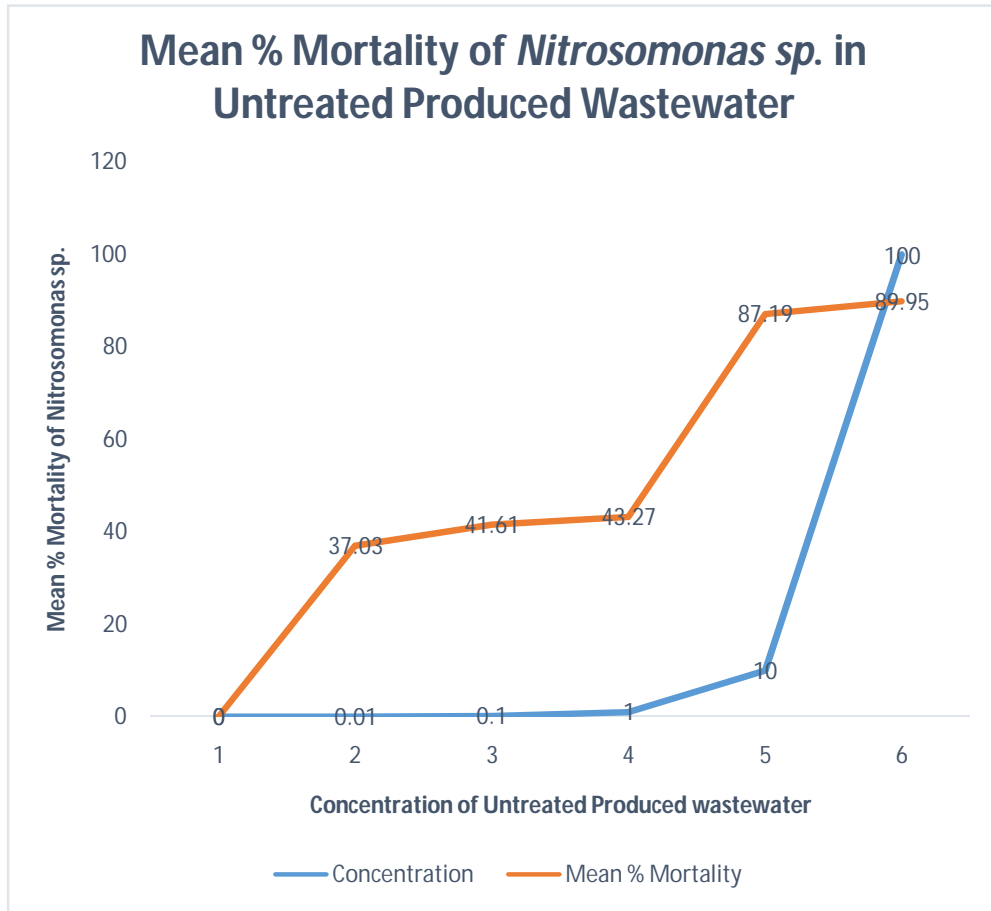
Fig 1: Mean percentage mortality of Nitrosomonas sp. exposed to untreated produced wastewater for 48 hours.
