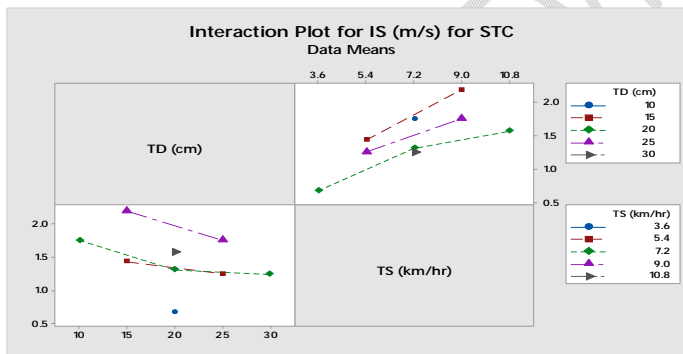
Fig. 5. Interaction plot of implement speed (m/s) for spring tine cultivator (STC) at the study location
