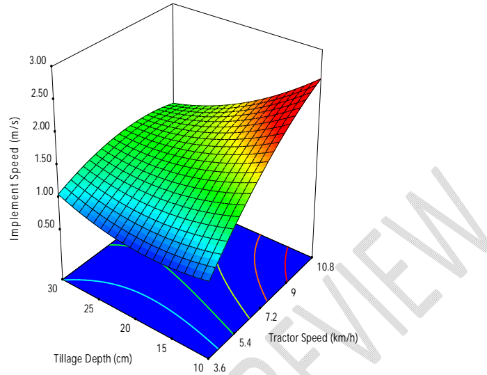
Fig. 3. Response surface plot of tillage depth and tractor speed against implement speed for ODH at the study location
