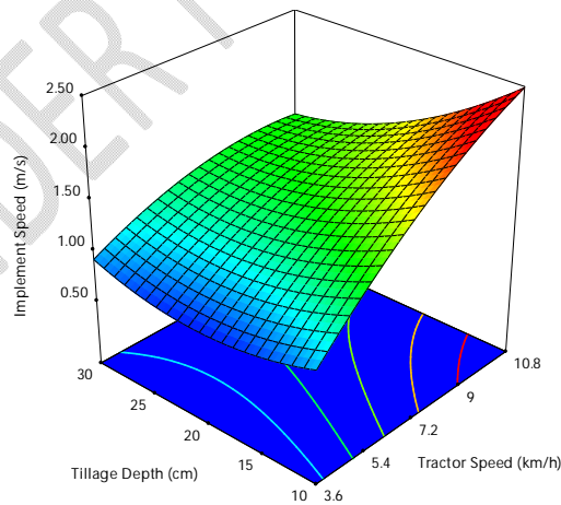
Fig. 2. Response surface plot of tillage depth and tractor speed against implement speed for STC at the study location
