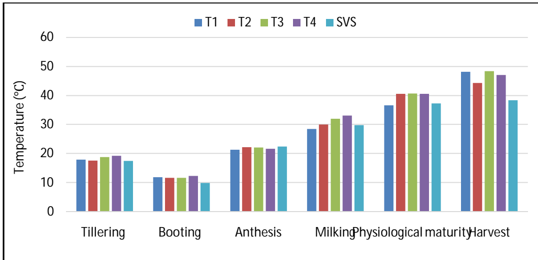
Fig.3. Canopy maximum temperature at various growth stages of wheat
