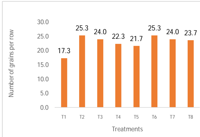
Fig 3: Effect of nano nitrogen on test weight
