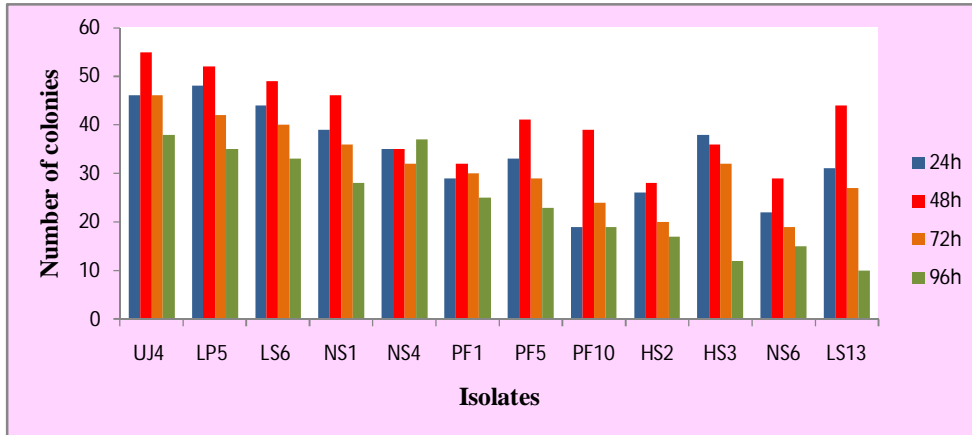
Effect of incubation period on the growth of selected bacterial isolates
