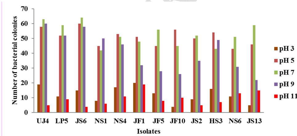
Effect of different pH on the growth of bacterial isolates
