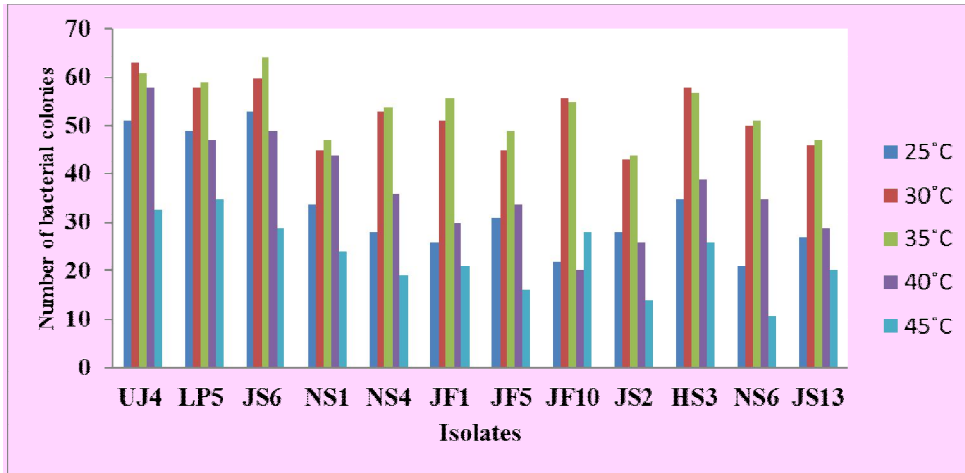
Effect of different temperature on the growth of selected bacterial isolates
