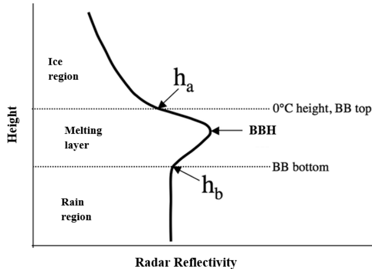
Figure 1: Illustration of the Vertical Profile of Radar Reflectivity
