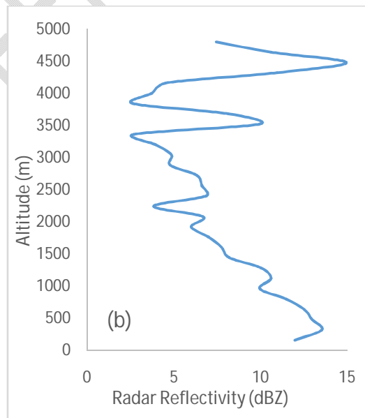
Figure 3: Vertical profile of radar reflectivity for; (a) a typical rainy day, September 21, 2010 (b) the average value of the rainy day
