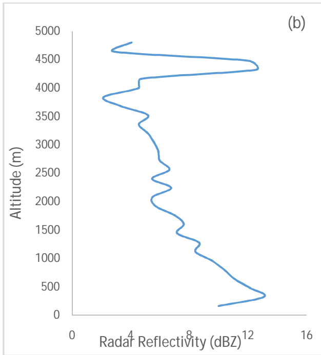
Figure 3: Vertical profile of radar reflectivity for; (a) a typical rainy day, September 21, 2010 (b) the average value of the rainy day
