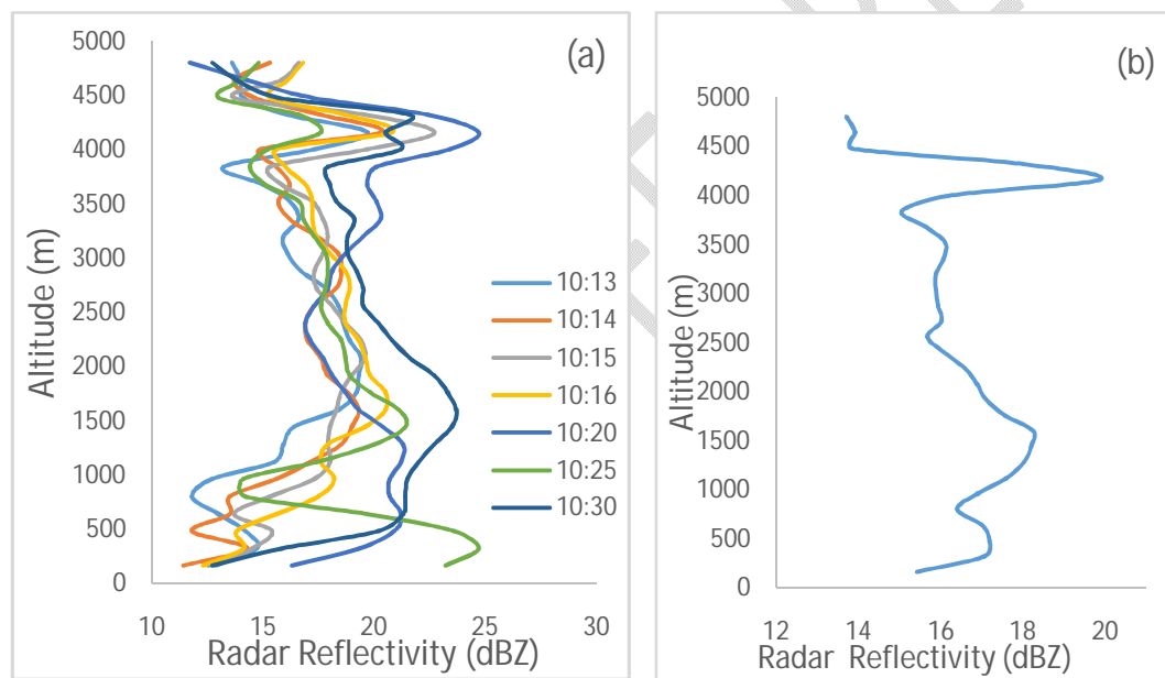
Figure 2: Vertical profile of radar reflectivity for; (a) a typical rainy day, September 3, 2010 (b) the average value of the rainy day
