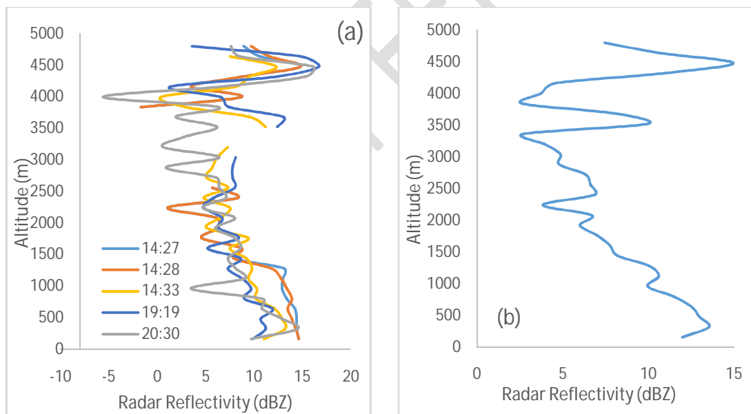
Figure 3: Vertical profile of radar reflectivity for; (a) a typical rainy day, September 21, 2010 (b) the average value of the rainy day
