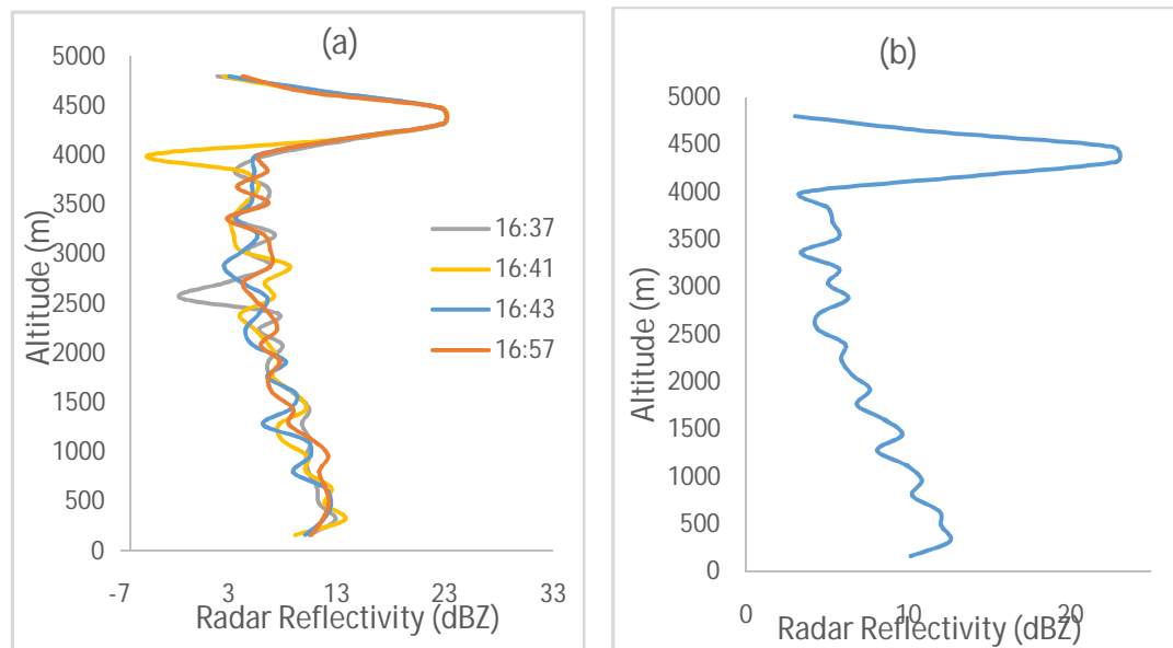
Figure 5: Vertical profile of radar reflectivity for; (a) a typical rainy day, October 28, 2010 (b) the average value of the rainy day
