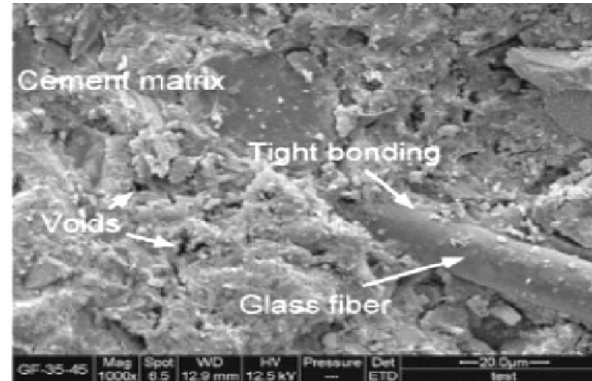
Fig. 9 SEM image of concrete with GF and micro silica
