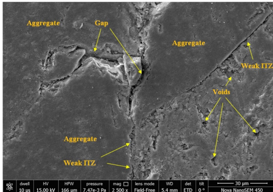
Fig. 8 SEM image of control mix
