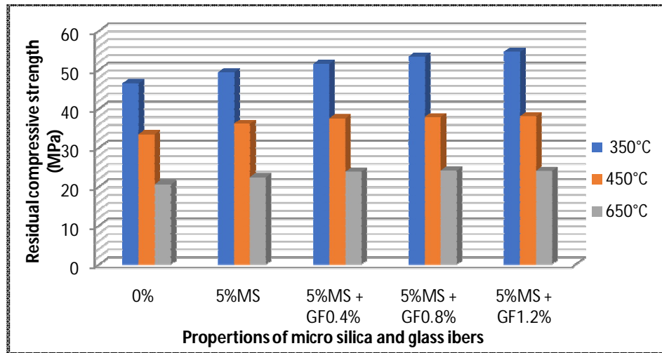
Fig. 7 Residual compressive strength of GFRC at elevated temperature
