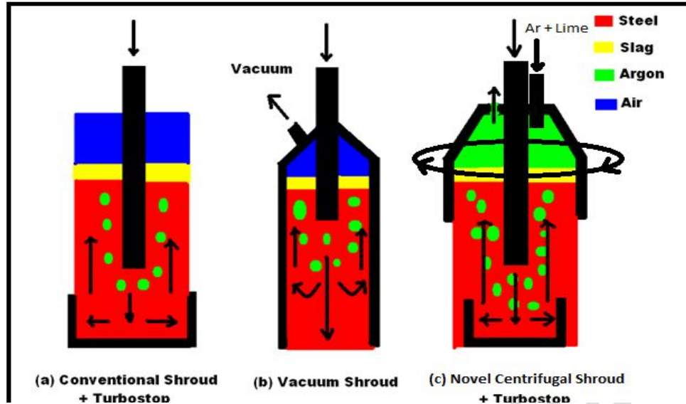
Fig. 4 Schematic of (a) Conventional Shroud and turbo-stop, (b) Vacuum Shroud with Argon Purging (Invented by Dr. Debasish Chatterjee) and (c) Novel Centrifugal Shroud (Invented Dr. Debasish Chatterjee)-Turbo-stop with Argon Purging
