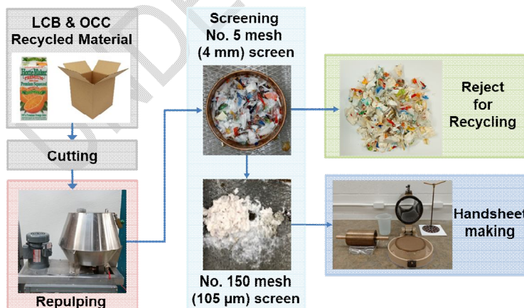
Fig. 3. Laboratory Repulping [30]
