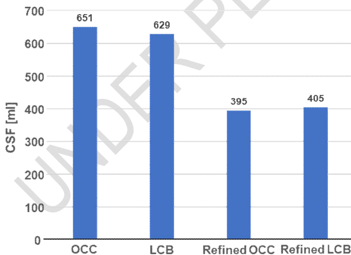
Fig. 4. CSF level of unrefined and refined OCC and LCB Fibers
