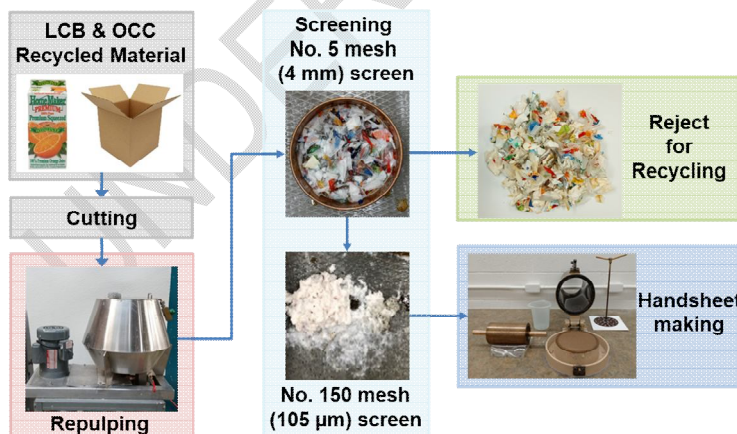
Fig. 3. Laboratory Repulping [30]
