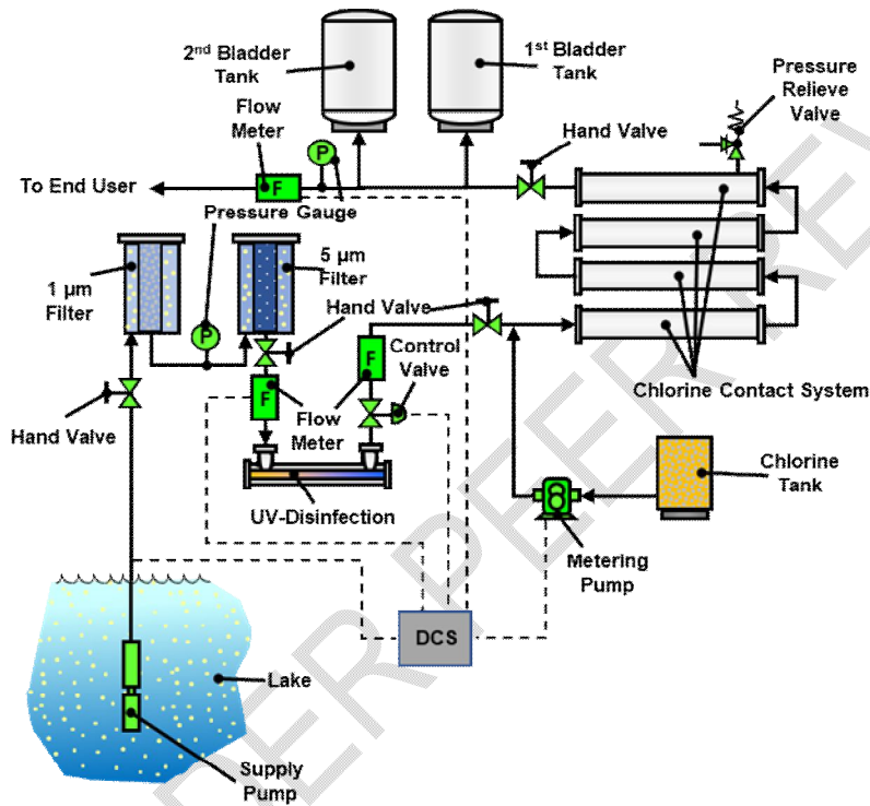
Fig. 2. System for the production of portable water [24]
