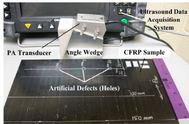
Figure 7. Experimental setup for flaw detection in CFRP sample using PAUT guided wave method
