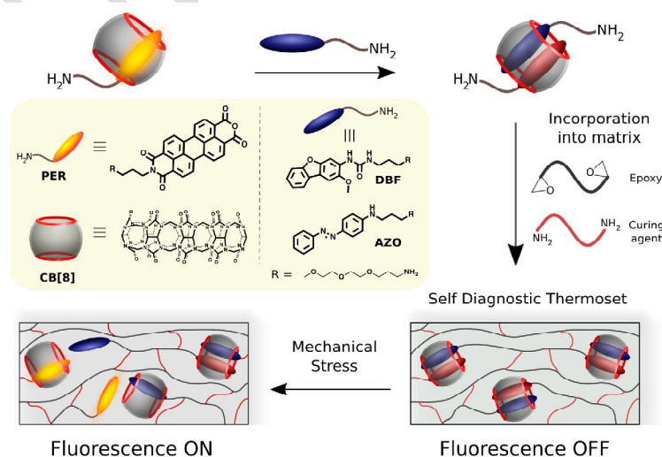
Figure 9. Schematic representation of the working principle and components of the damage reporting carbon fiber-epoxy resin composites
