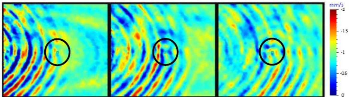
Figure 1. Interaction of the A0 mode with the damage from the high-resolution scan at 100 kHz with area of damage circled
