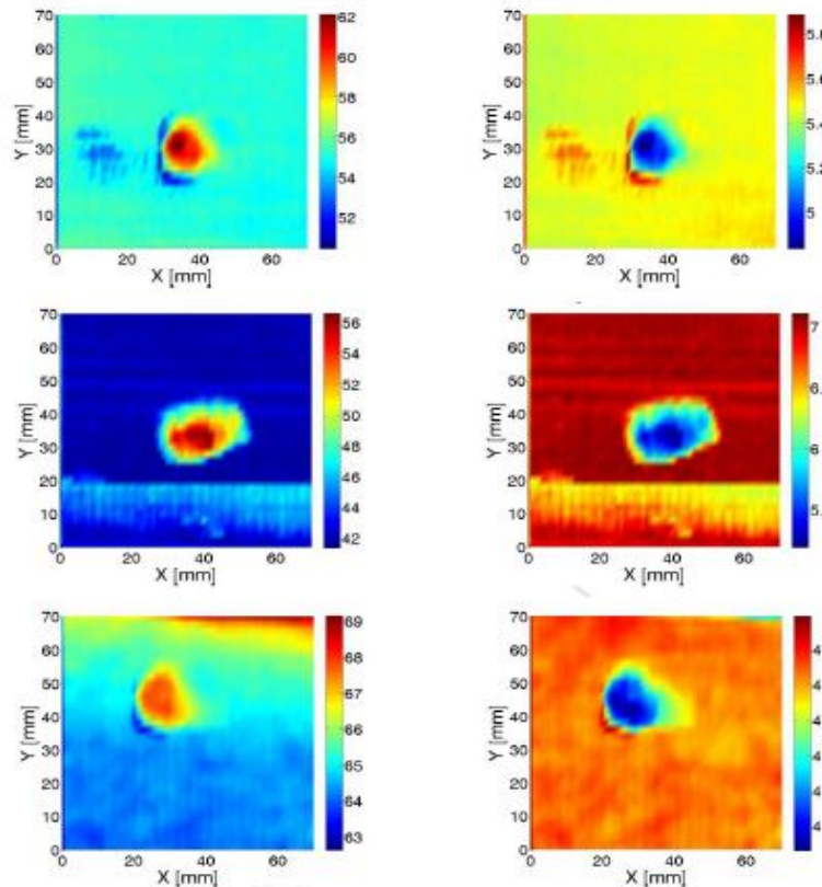
Figure 2. Capacitive images of delamination due to impact in the CFRP samples acquired at 300.04MHz, capacitance
