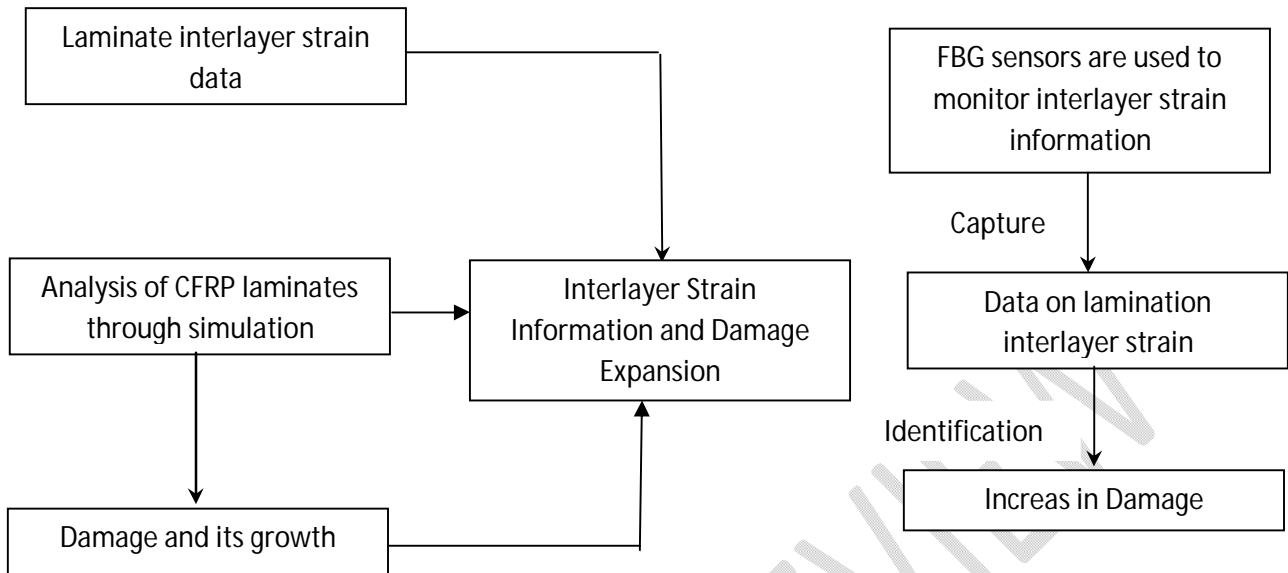
Figure 5. Damage recognition theory based on FBG Sensor for CFRP laminated plates
