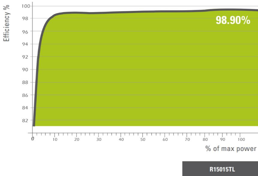
Figure 4.12. Efficiency curve FIMER – Model: R15015 TL central inverter
