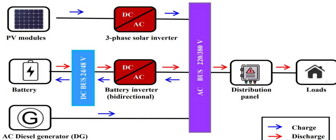
Figure 4.3 solar plant schematic diagram for omorate mini off-grid site
