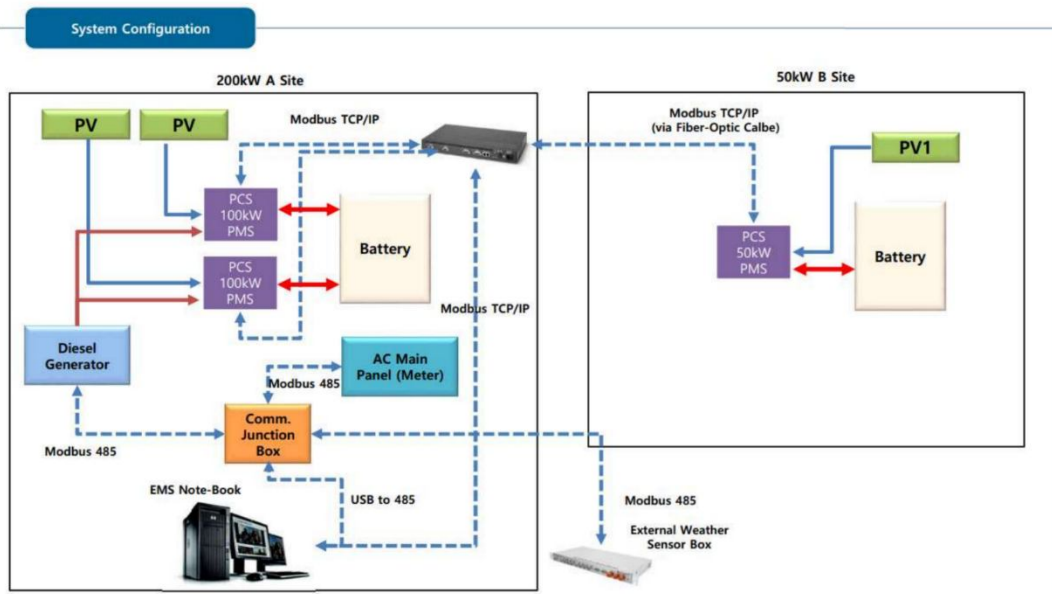
Figure 4.6. The schematic diagram of koftu solar power site.
