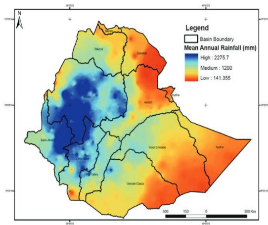
Figure 2.3 mean annual Rainfall (mm) [31]
