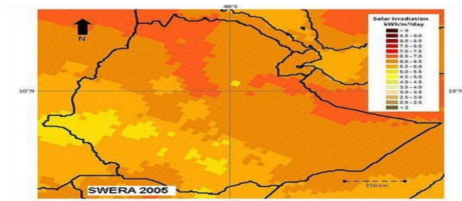
Figure 2.3 Solar radiation in Ethiopia in (kWh/m 2 /day)[27]
