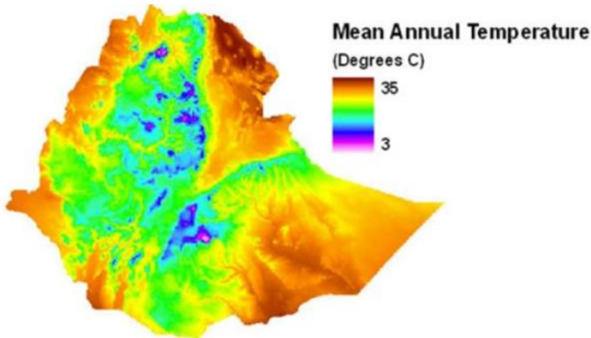
Figure 2.2 Mean annual temperature [29]
