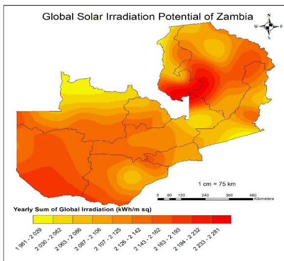
Figure 2. 5 Annual Total Global Solar Radiation Intensity source: [36]
