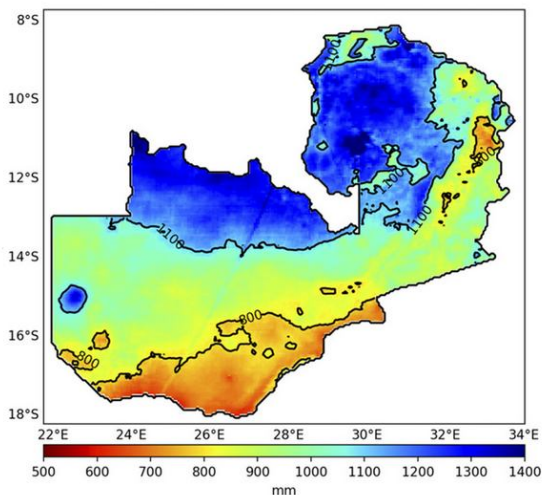
Figure 2.7 average annual rainfall map of Zambia, 2000-16, source: CHIRPS [40]
