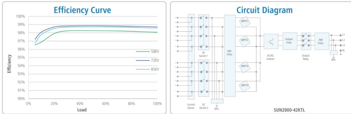
Figure 4.9. Smart String Inverter SUN2000-42KTL circuit diagram and efficiency curve
