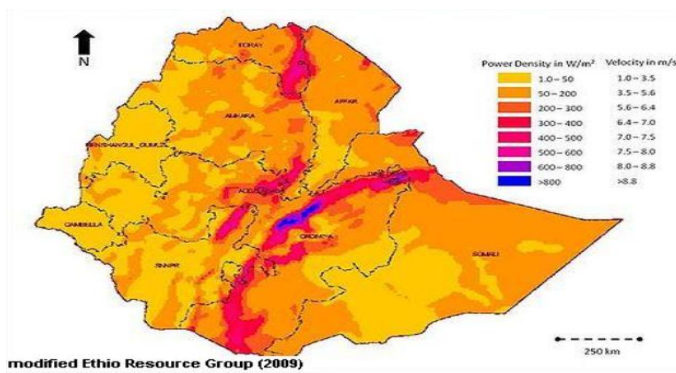
Figure 2.4 annual mean wind power density in W/M^2 and velvety in m/s [33]
