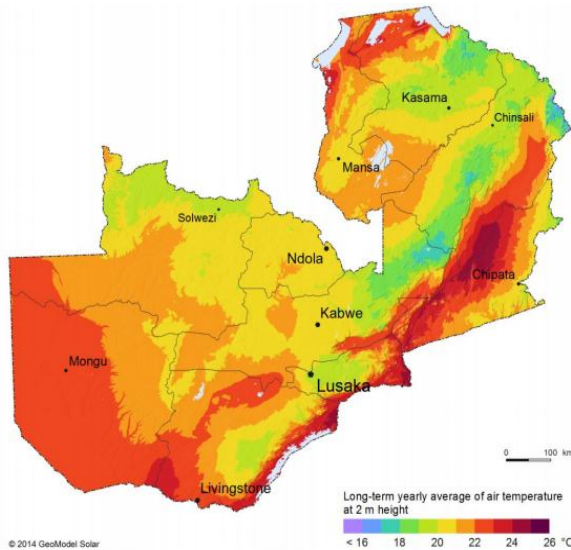
Figure 2.6 Long term yearly average of air temperature at 2 meters. Source: CFSR
