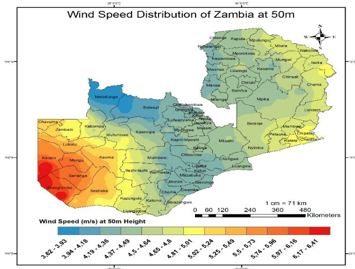
Figure 2.8 Annual Wind Speed at 50m [42]
