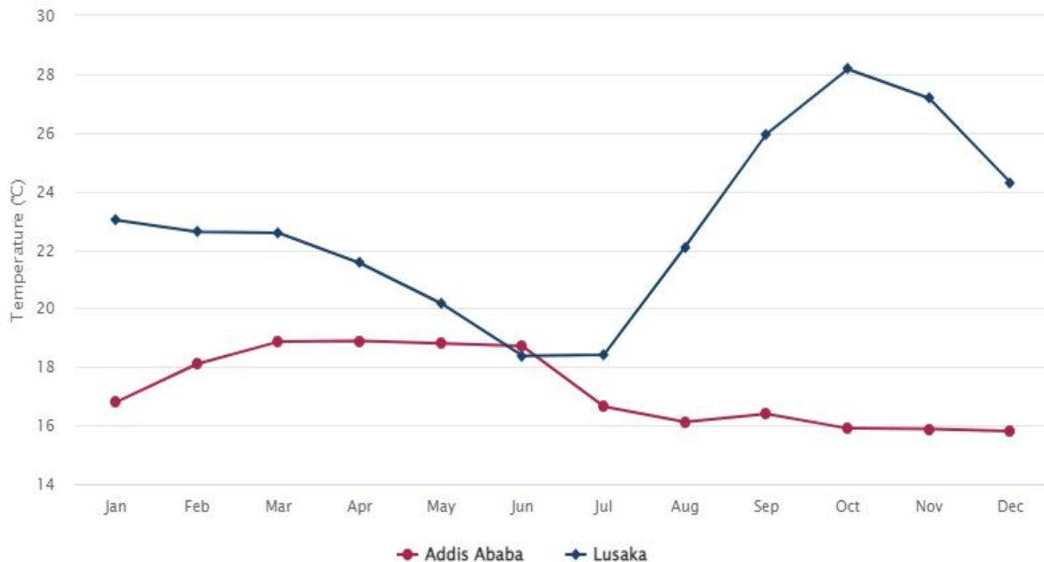
Figure 4.14. compare the average annual temperature Addis Ababa the capital city of Ethiopia and Lusaka the capital city of Zambia. [54]
