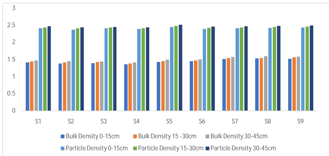
Fig 1: Bulk density and Particle density (Mg m -3 )
