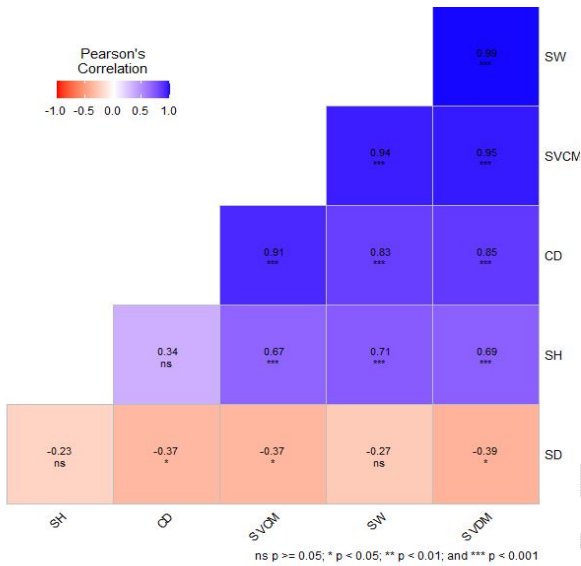
Figure 3. Correlation between various stalk traits viz., SH, CD, SVCM, SW, SVDM. ** denotes significant at 1%, * denotes significant at 5%, and ns denotes non-significant. The intensity of the colour indicates the strength of the correlation.
