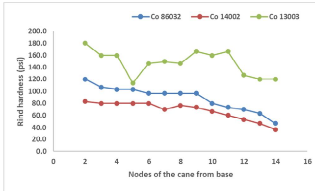
Figure 5: Comparison of rind hardness of sugarcane clones based on the soil penetrometer
