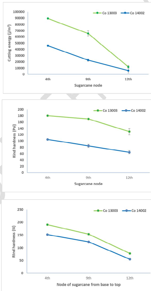
Figure 5: Comparison of rind hardness of sugarcane clones based on the soil penetrometer
