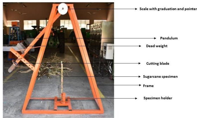
Figure 1. Pendulum-type impact test rig
