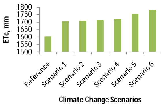
Fig. 3. Crop water requirement of Mulberry at (a) Shorapur, (b) Shahapur, and (c) Yadgir
