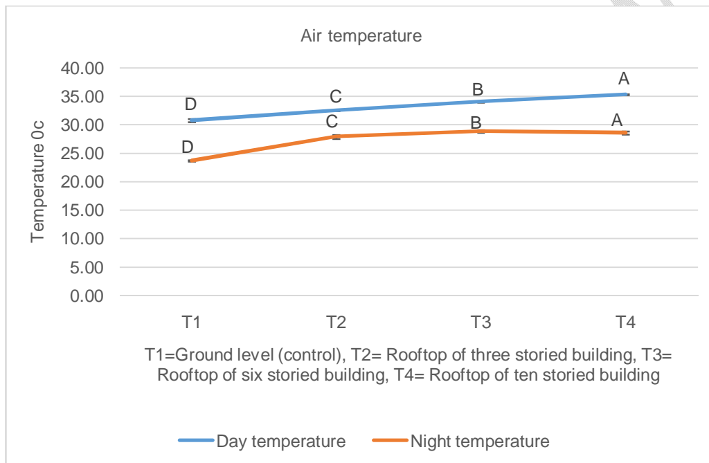
Figure 1. Day and Night air temperature at different building height of rooftop garden
