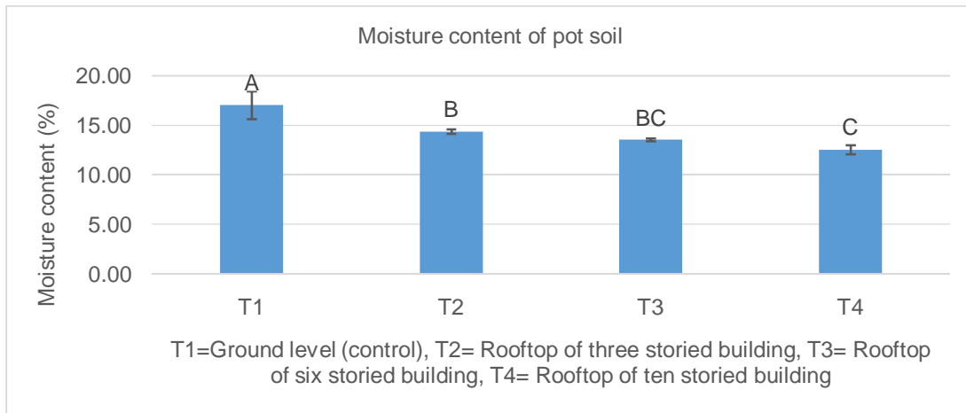
Figure 2. Moisture content of pot soil at different building height of rooftop garden
