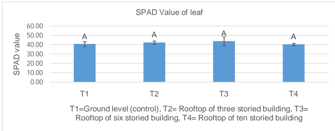
Figure 3. SPAD value of tomato at different building height of rooftop garden
