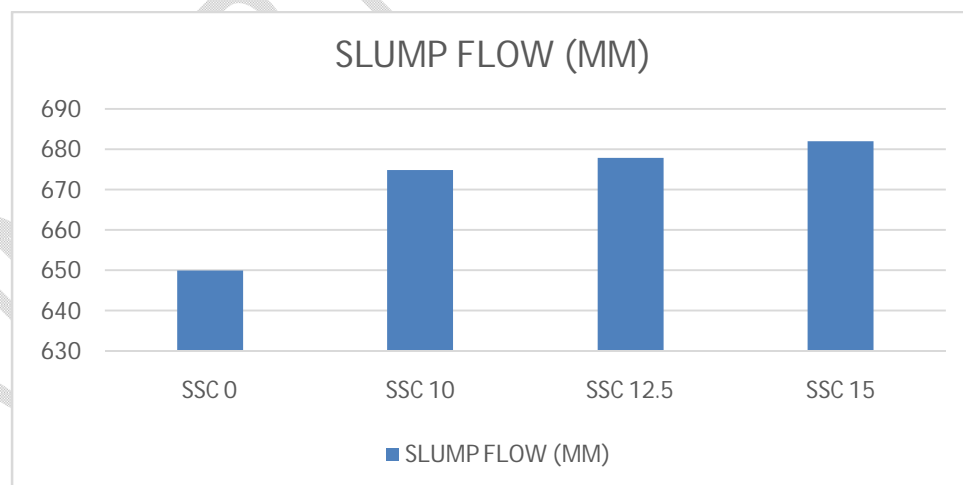
Fig. 1. Slump flow in mm [12]
