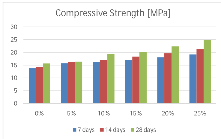
Fig. 10. Compressive strength results [22]
