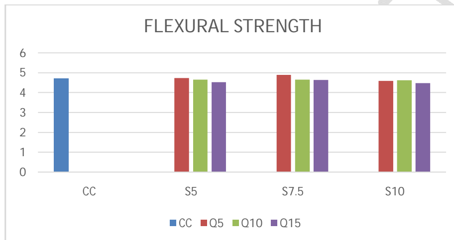
Fig. 13. Flexural strength test results [25]
