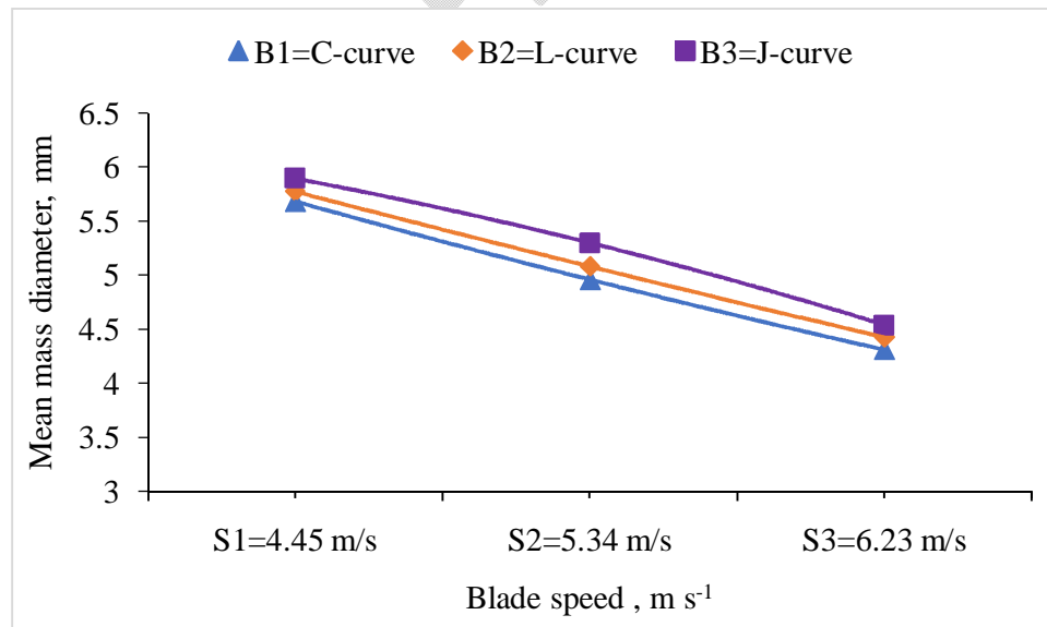
Fig .3: Interactive effect of blade speed and blade type (S×B) on mean mass diameter
