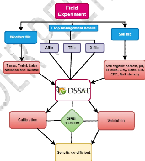
Fig 1 Methodology of DSSAT-CERES module
