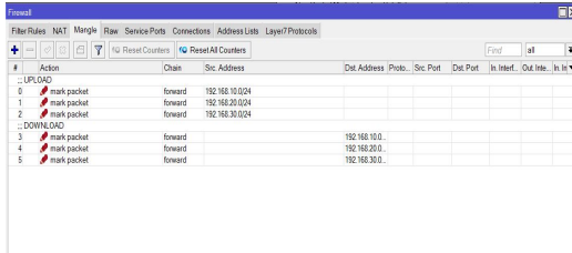
Fig.6 Mangle List Uploaddan Download
