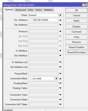
Fig.2 Configure Mangle Uploads
