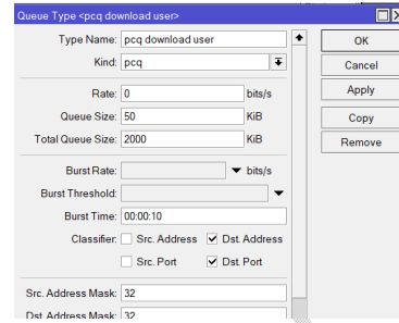
Fig.8 Download PCQ Configuration
