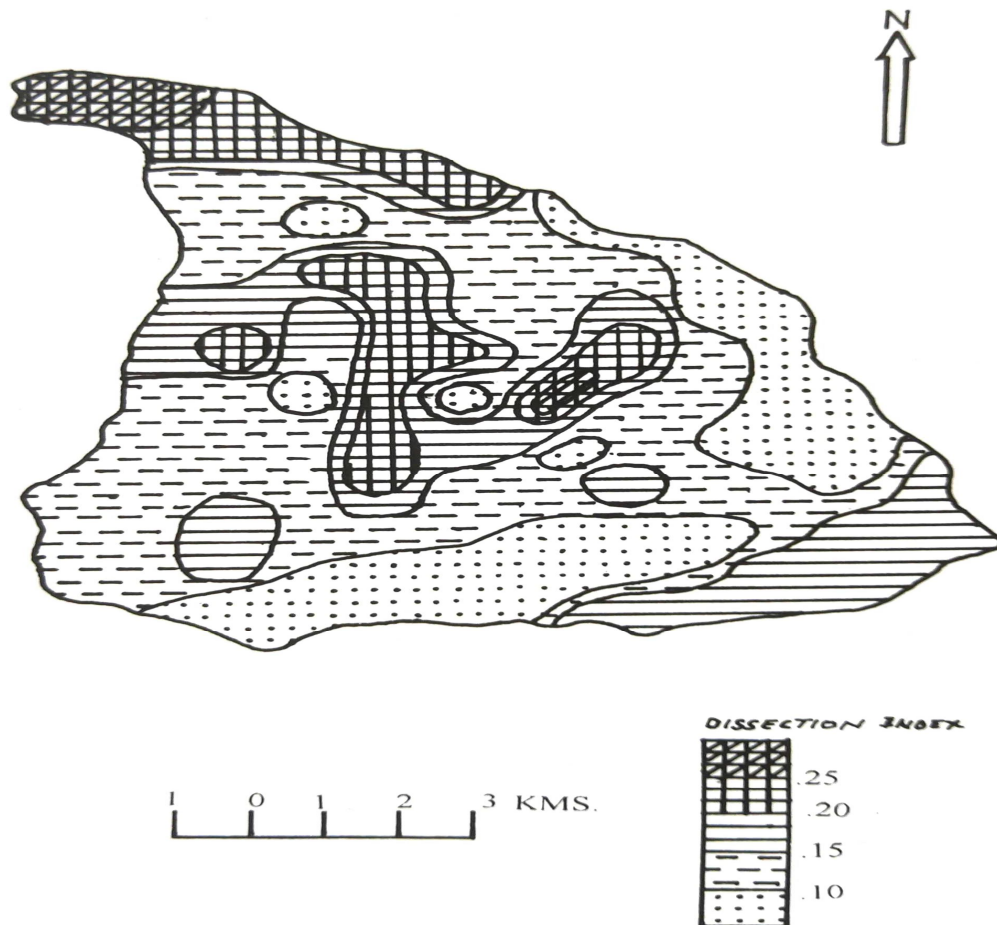
Fig.7. Dissection Index of Watershed
