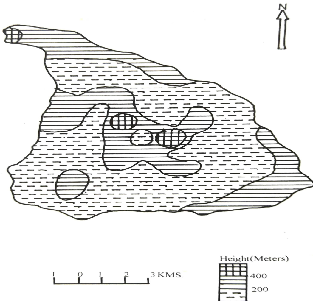
Fig.5. Relative Relief of Watershed
