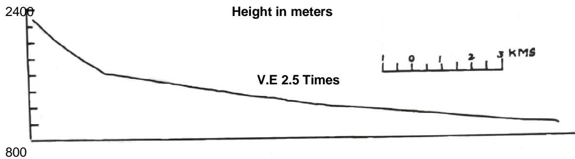
Fig.12. Longitudinal Profile of Area
