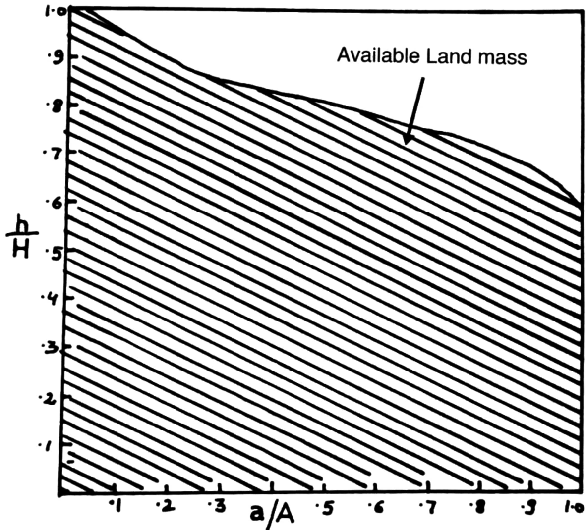
Fig.9. Hypsometric Curve of Watershed
