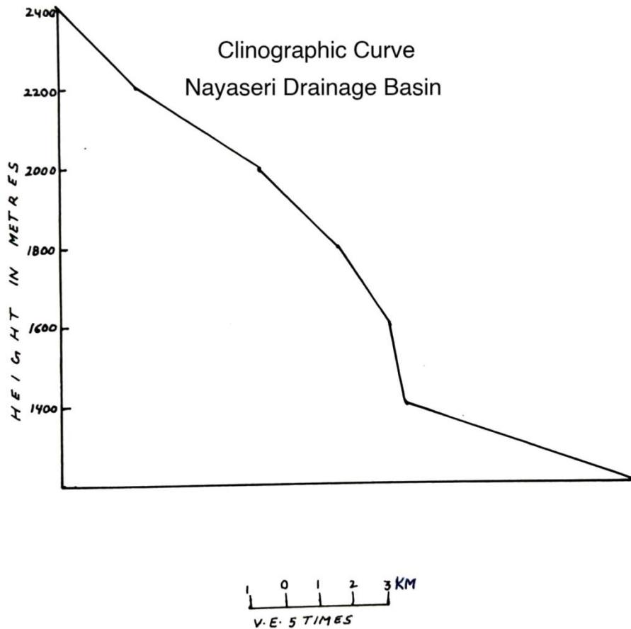
Fig.10. Clinographic Curve of Watershed
