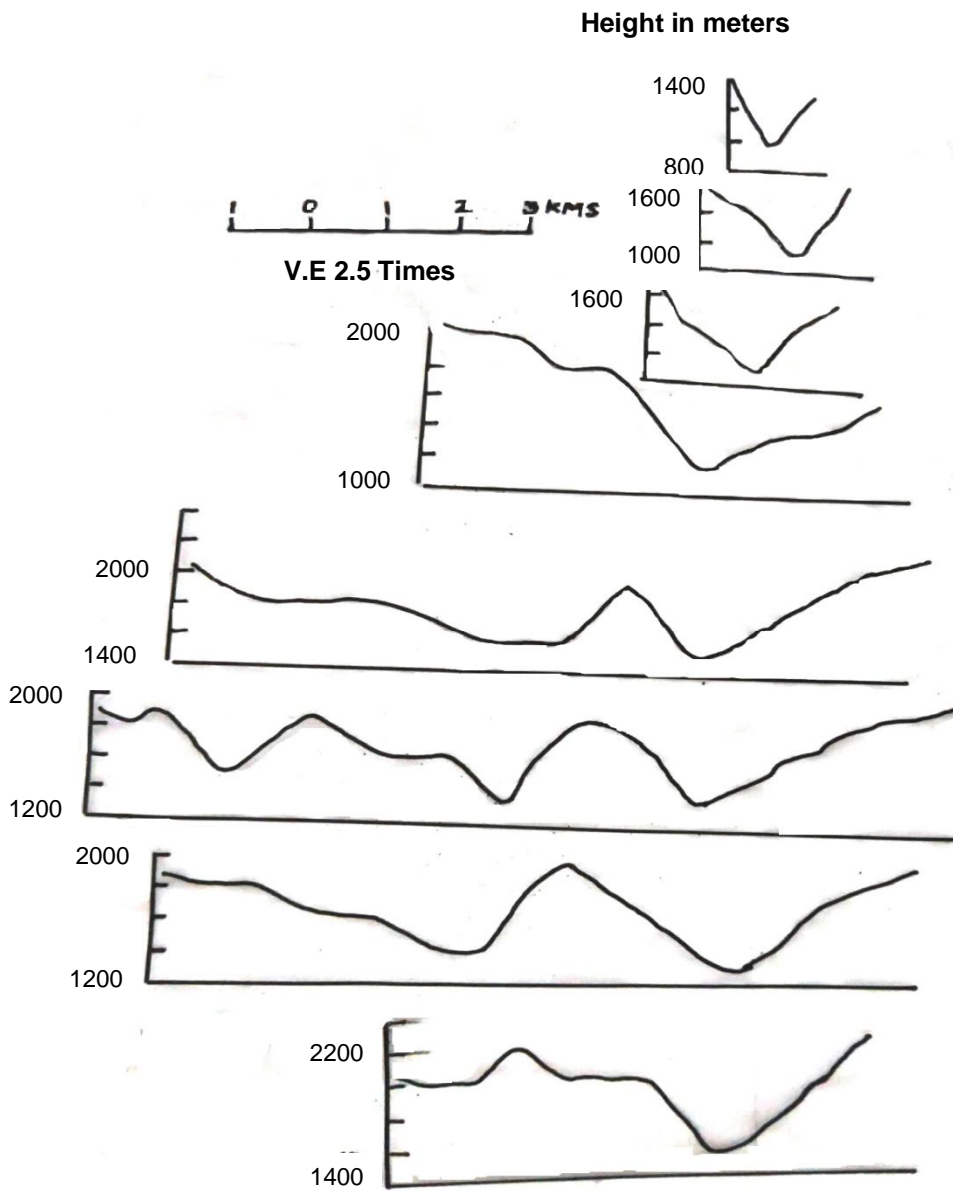
Fig.11. Relief Profile (Cross Section)
