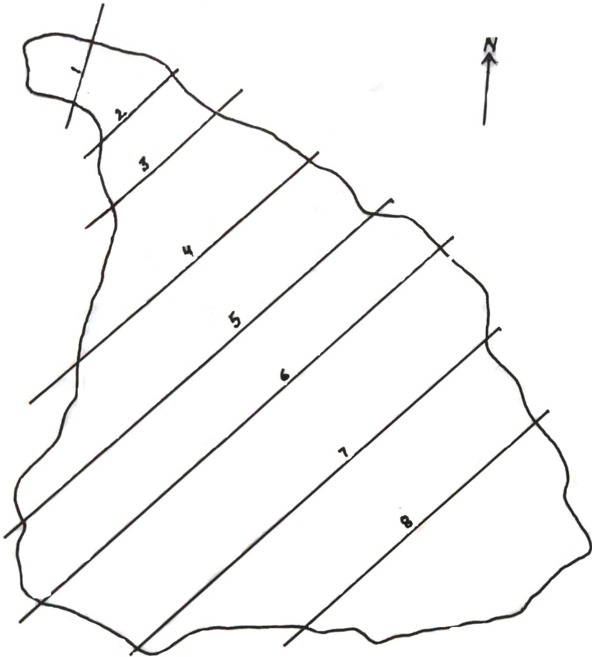
Fig.11A. Section Lines on Map
