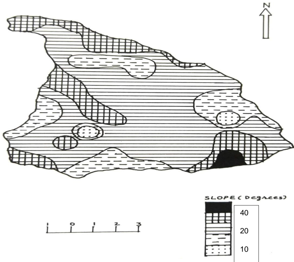
Fig.6. Average slope of Watershed
