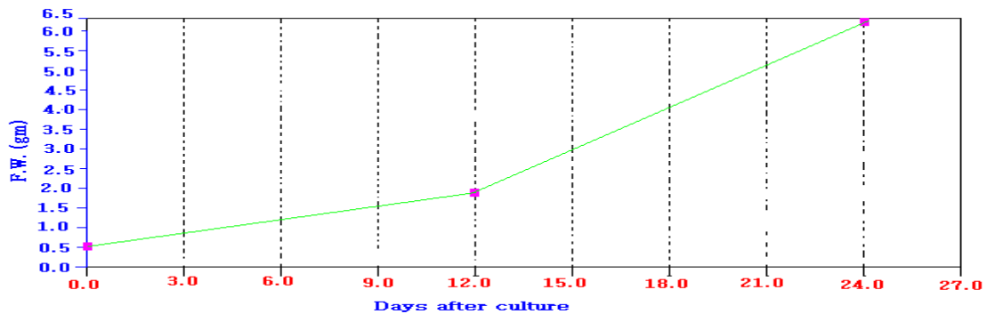
Fig. 3. Growth curve of suspension cultures of Ginkgo biloba grown in the MS medium supplemented with 2.0 mg/l Pb for 24 days.
