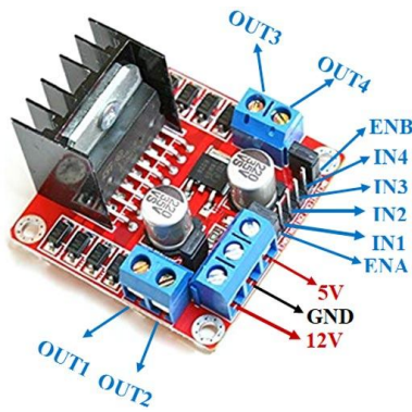
Fig. 10. L298N Motor Driver
