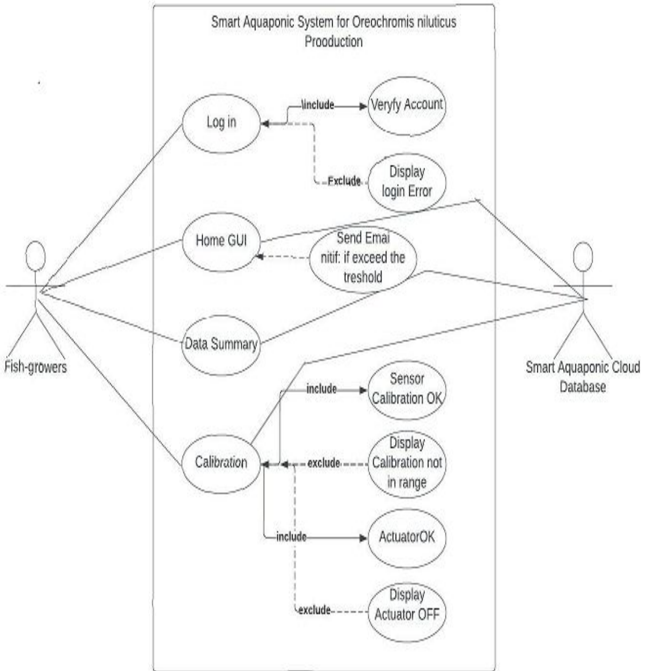
Figure 25 - Use Case Diagram
