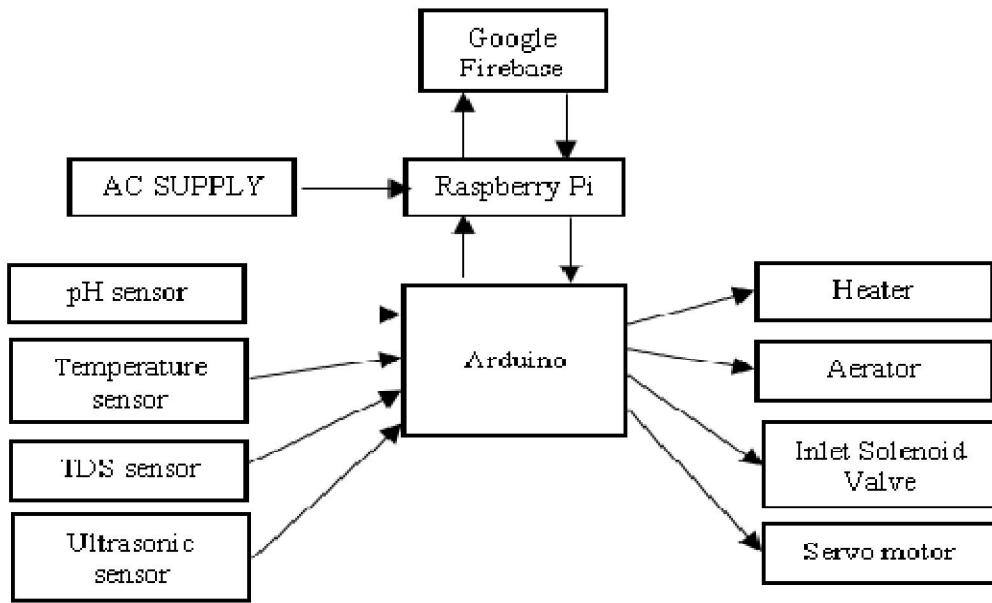
Figure 2 - Block Diagram of the Project
