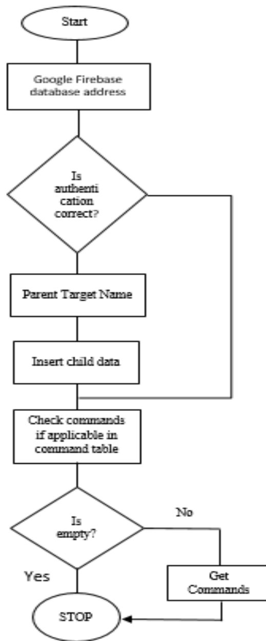
Figure 24 - Flowchart of the Web-based Design
