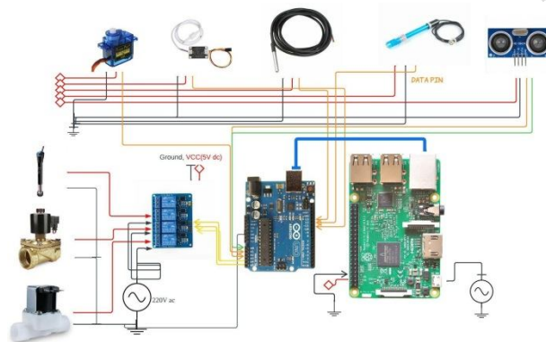
Figure 16 - Schematic Diagram
