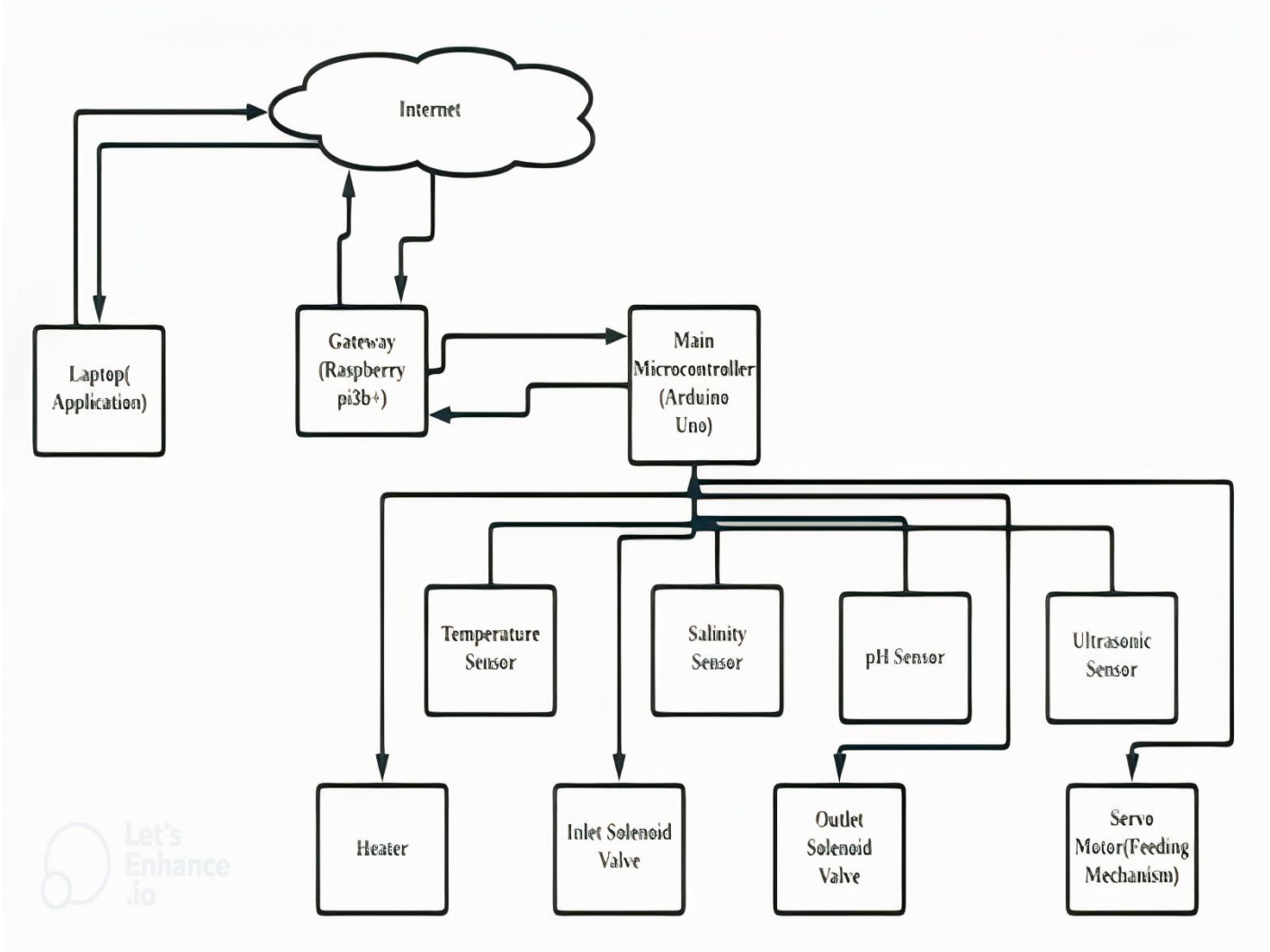
Figure 23 – Set - Up Diagram
