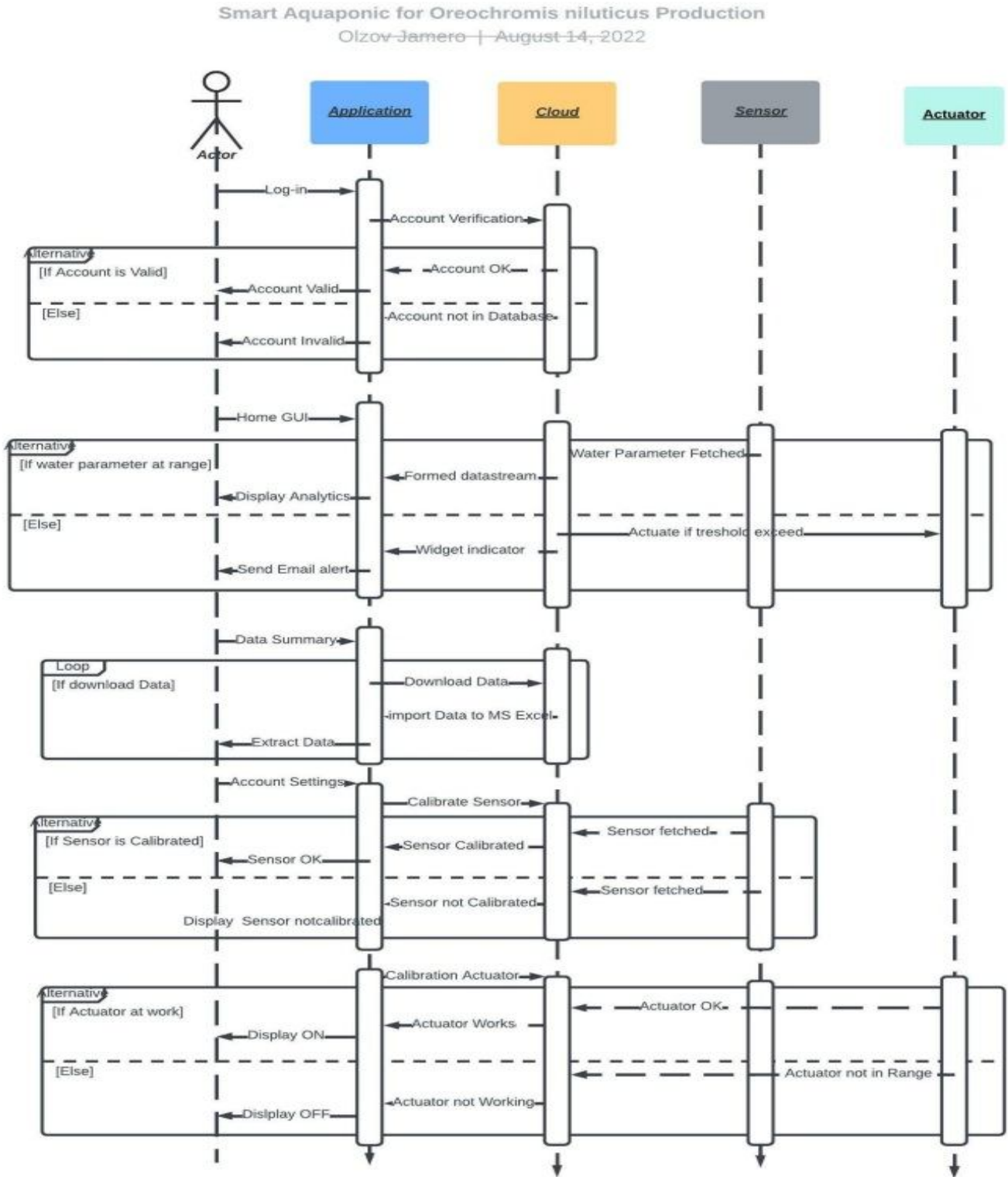
Figure 26 - Sequence Diagram
