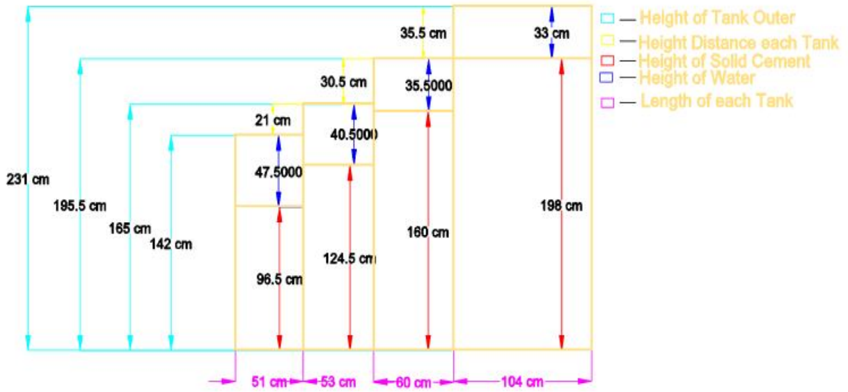
Figure 20 - Dimensions of the Tank
