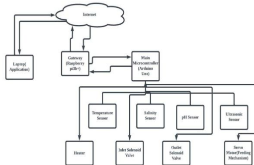
Figure 23 - Set - Up Diagram
