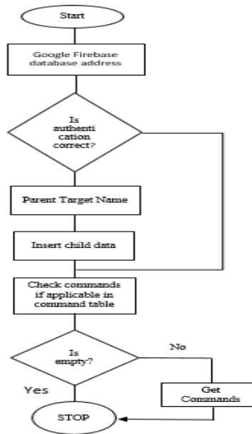
Figure 24 - Flowchart of the Web-based Design
