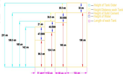
Figure 20 - Dimensions of the Tank
