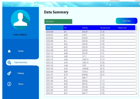
Figure 29 - Software Data Summary
