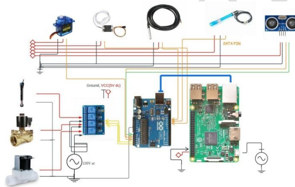
Figure 16 - Schematic Diagram
