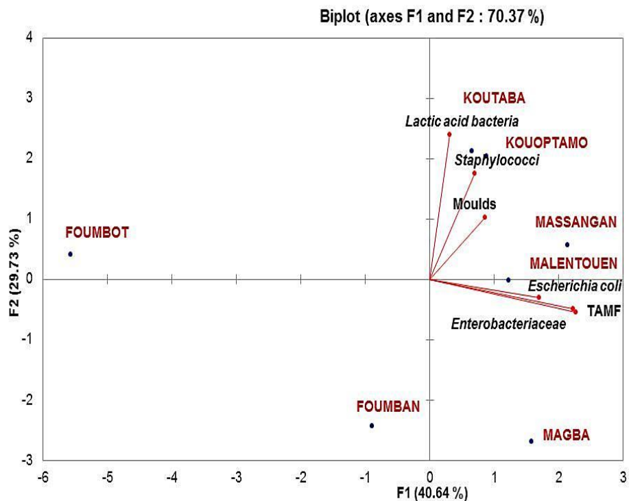
Fig. 7: Projection of observations and variables on the axis system F1xF2
